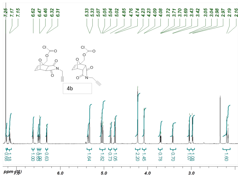
Figure S11. ^1\text{H} NMR spectrum of Chloroformate 4b ( \text{CDCl}_3 , 400Hz).
