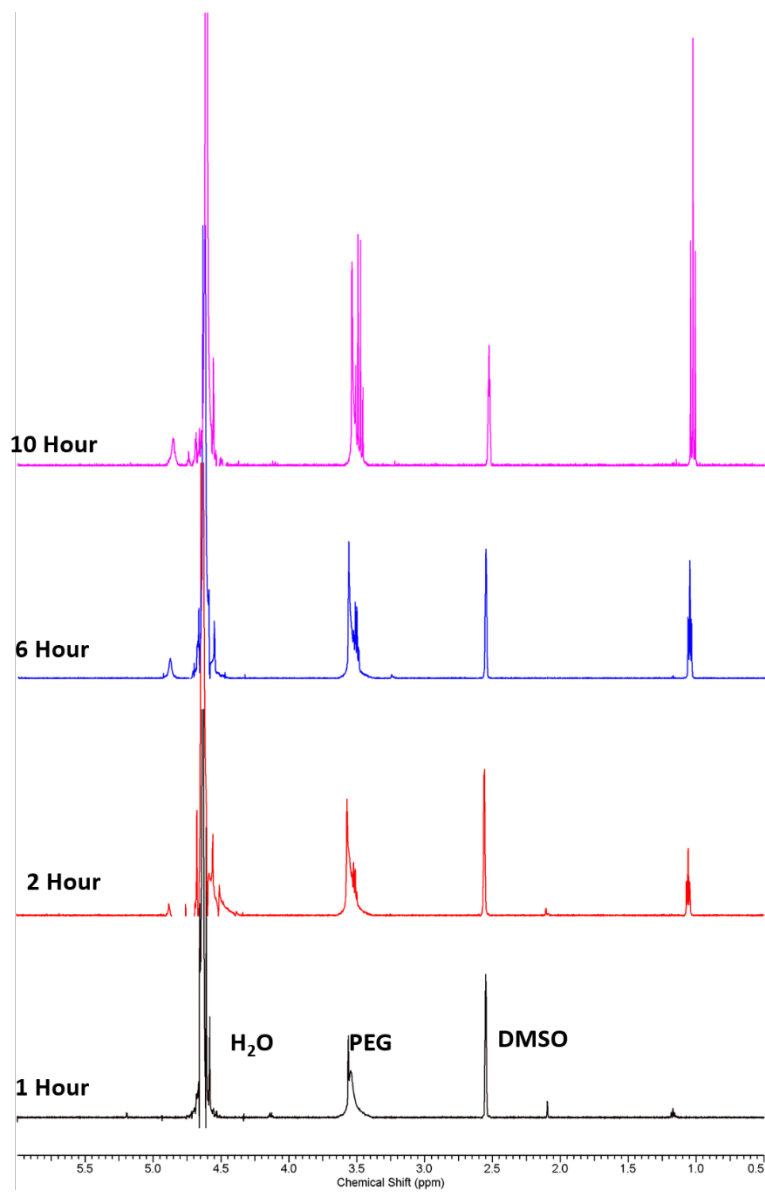
Figure S27. 1 H NMR spectra of Micelle-control incubated in 5:1 DMSO- d 6 :D 2 O at 75 °C.
