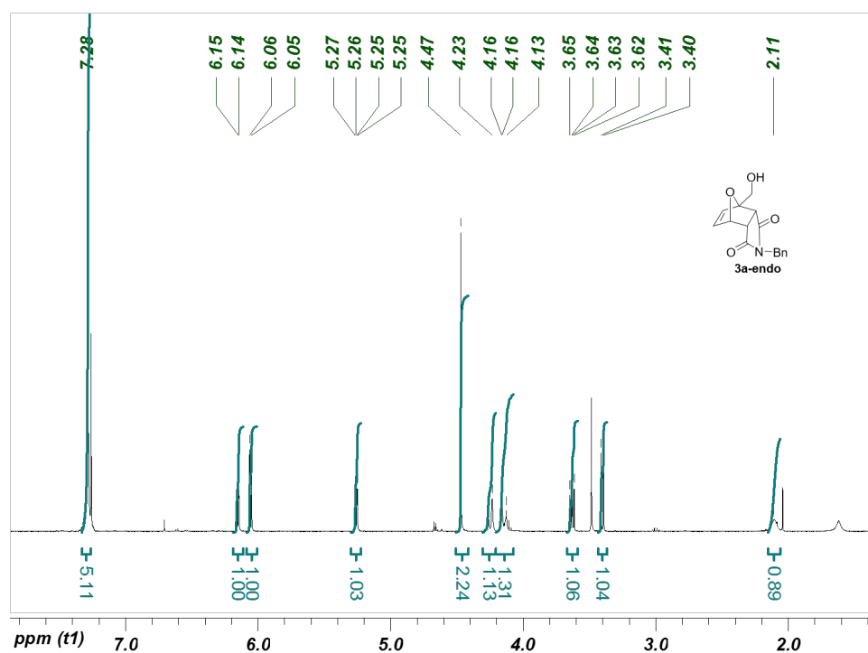
Figure S1. 1 H NMR spectrum of Compound 3a-endo (CDCl 3 , 600Hz).
