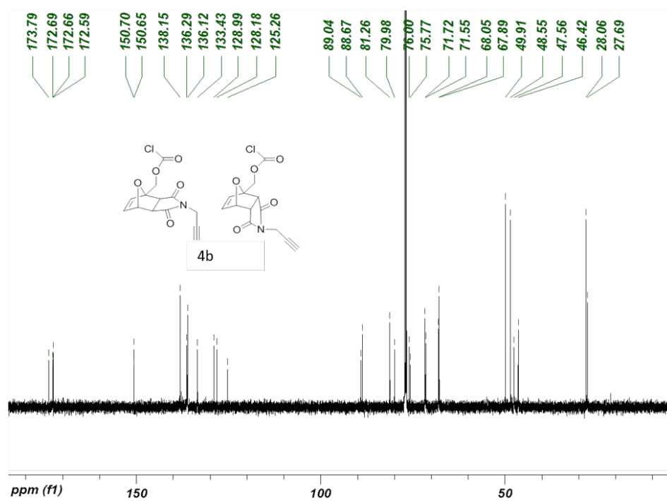
Figure S12. ^{13}\text{C} NMR spectrum of Chloroformate 4b ( \text{CDCl}_3 , 100Hz).
