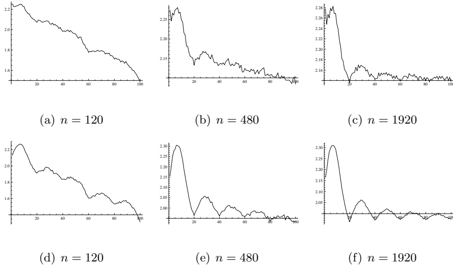
Figure 3: Model M1 : logarithms of the upper quantiles of simultaneous confidence intervals for \Re a(\lambda, 0) (first row) and for \Im a(\lambda, 0) (second row), \lambda \in \bar{\Lambda} for cEMBB. On the horizontal axis block length b \in \{1, 2, \dots, 100\} .
