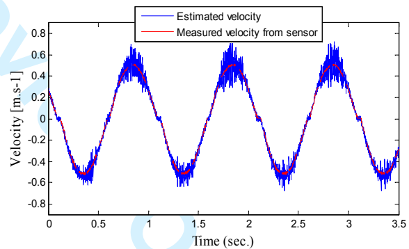
Figure 8. Velocity [m.s-1]: estimated by CBD.
