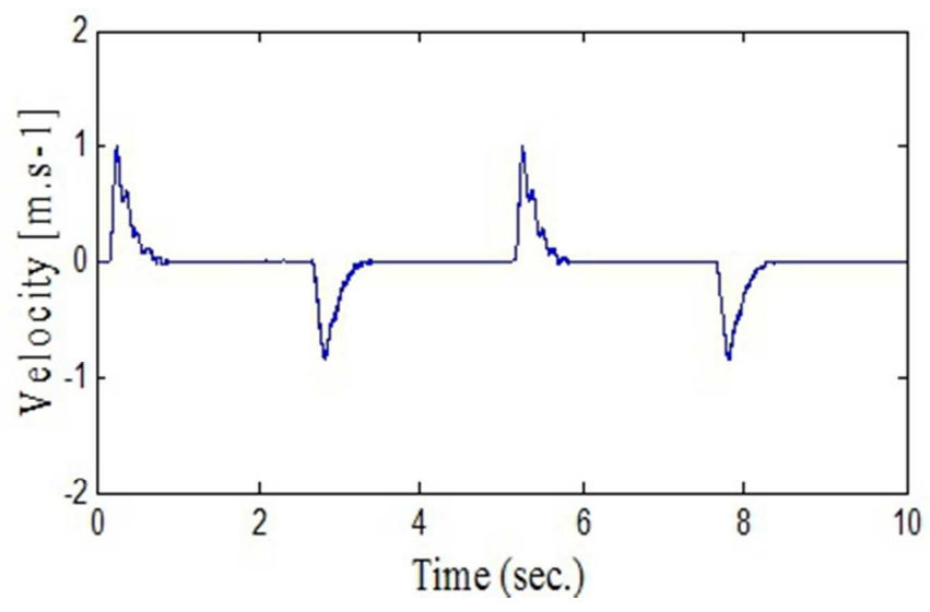
Figure 16. Velocity [m.s-1]: with PD.
