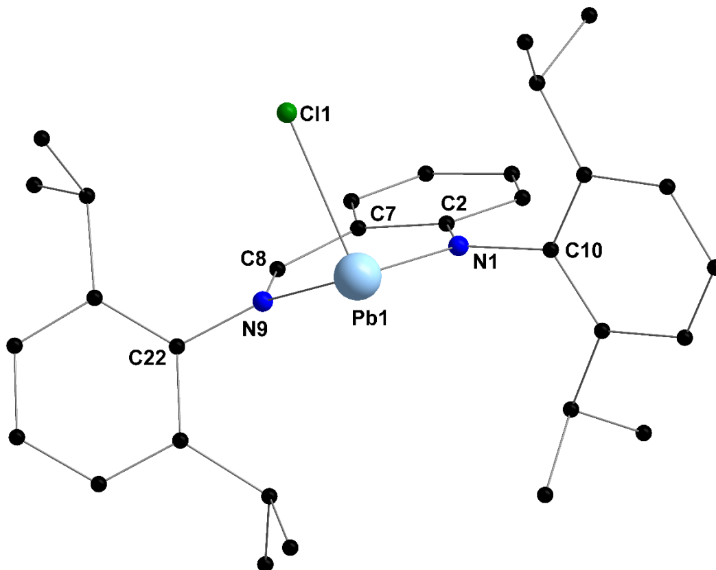
Figure 2: Molecular solid-state structure of one of the two independent components ( 1a ) in [\{N^{iPr}\}PbCl] ( 1 ). H atoms are omitted for clarity. Selected interatomic distances (Å) and angles (deg): Pb1-N1 = 2.246(6), Pb1-N9 = 2.336(6), Pb1-Cl1 = 2.5912(19), N1-C2 = 1.357(9), N1-C10 = 1.449(9), C2-C7 = 1.434(10), C7-C8 = 1.421(9), C8-N9 = 1.309(9), N9-C22 = 1.434(9); N1-Pb1-N9 = 80.60(2), N1-Pb1-Cl1 = 94.60(16), N9-Pb1-Cl1 = 84.98(15), C2-N1-C10 = 119.50(6), C2-N1-Pb1 = 131.80(5), C10-N1-Pb1 = 108.60(4), C8-N9-C22 = 118.60(6), C8-N9-Pb1 = 125.20(5), C22-N9-Pb1 = 115.70(4). Pb1 sits 0.53 Å above the N1-C2-C7-C8-N9 mean plane.
