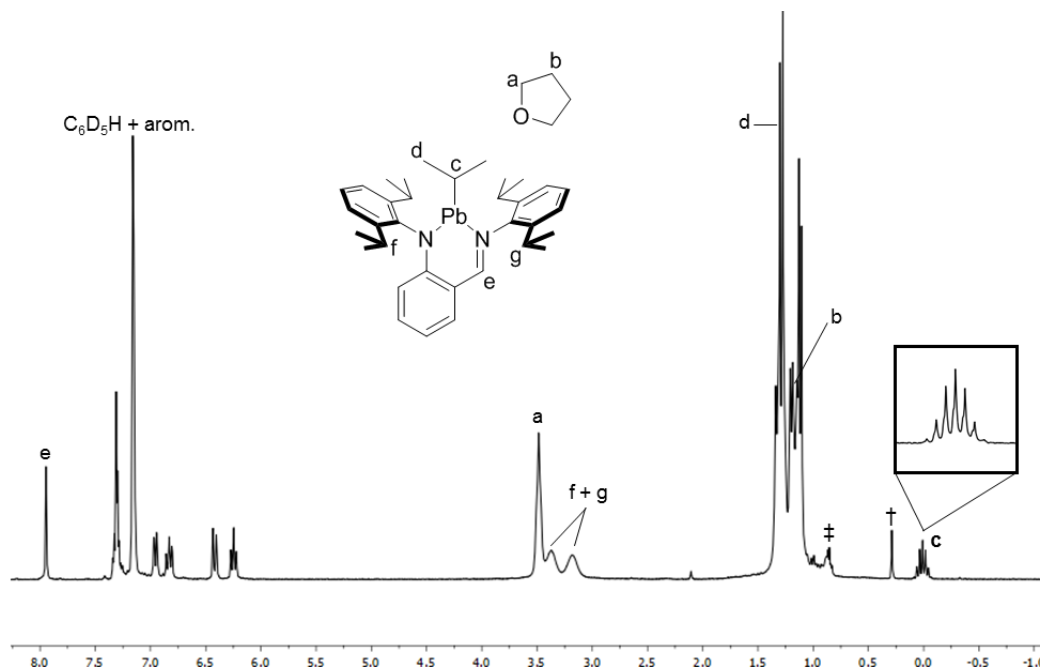
Figure 4: ^1\text{H} NMR spectrum (benzene- d_6 , 400 MHz, 298 K) of [\{\text{N}^{\text{iPr}}\text{N}\}\text{Pb}^{\text{iPr}}] ( 3 ). † = silicone grease. ‡ = residual pentane.
