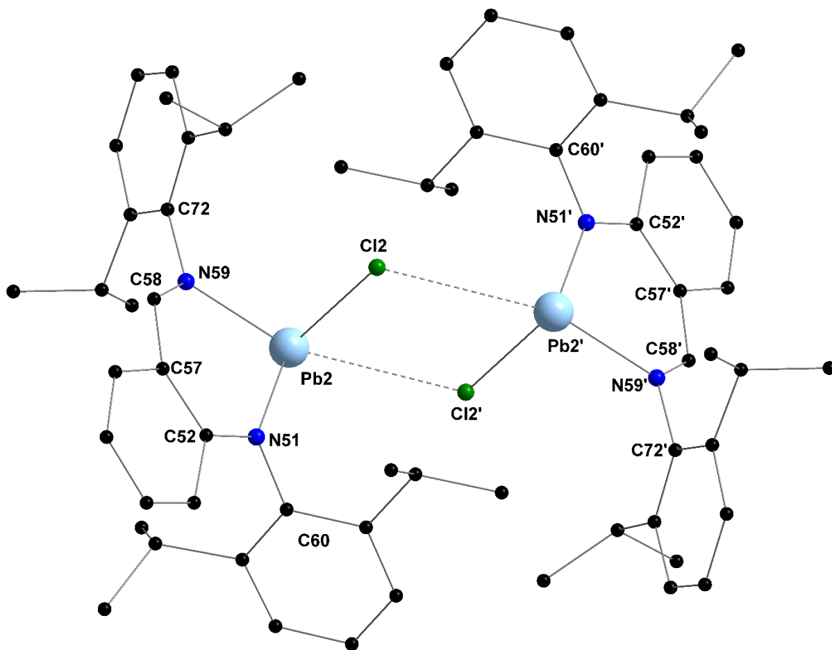
Figure 3: Representation of the molecular solid-state structure of one of the two independent components ( 1b ) in [\{N^iPr\}PbCl] ( 1 ), showing the short Pb2 \cdots Cl2' and Pb2' \cdots Cl2 distances with the symmetry-related 1b' . Selected interatomic distances (Å) and angles (deg): Pb2-Cl2 = 2.574(2) , Pb2-Cl2' = 3.353(2) ; Cl2-Pb2-Cl2' = 78.09(6) . See table 1 for other key parameters.
