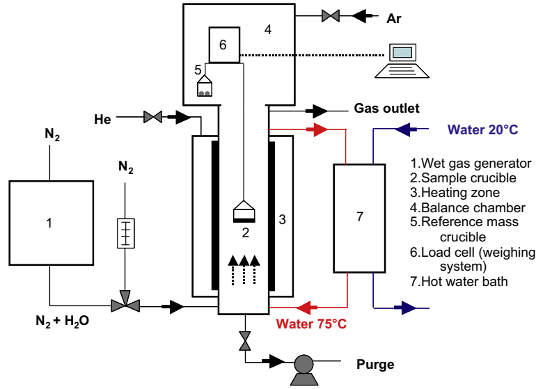
Fig. 1. Scheme of the TGA facility.
