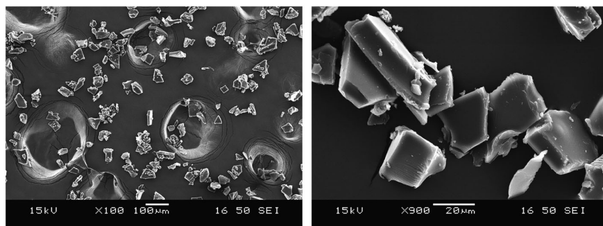
Figure 4. SEM images of ground S 110/6/250/6 extrudate ( d_p < 0.06 \mu\text{m} ). The larger circular spots belong to the adhesive tape.
