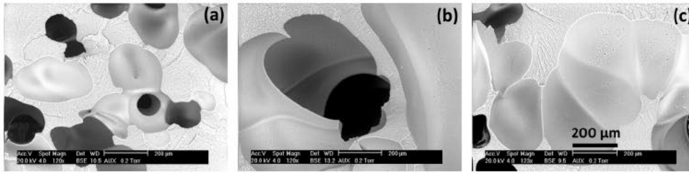
Fig. 9. SEM pictures for neat PHBV foams at various die temperature T_f , (a) 120 °C, (b) 130 °C, (c) 140 °C.
