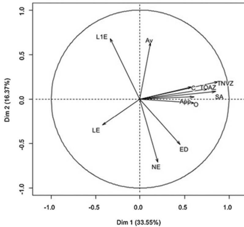
Figure 4. PCA realized with 11 behavioural variables of the three tests (cross-maze test, dyadic test, restraint test). For cross-maze test: LE: Latency to Emerge from the acclimatization zone, NVZ: Number of Visited Zones, TOAZ: Time spent Outside of the Acclimatization Zone, A: Activity; for dyadic test: App: Approach, O: Orientation, Av: Avoidance, C: Contact; and for restraint test: NE: Number of Escape attempt, ED: total Escape Duration, L1E: Latency before the first Escape attempt.
