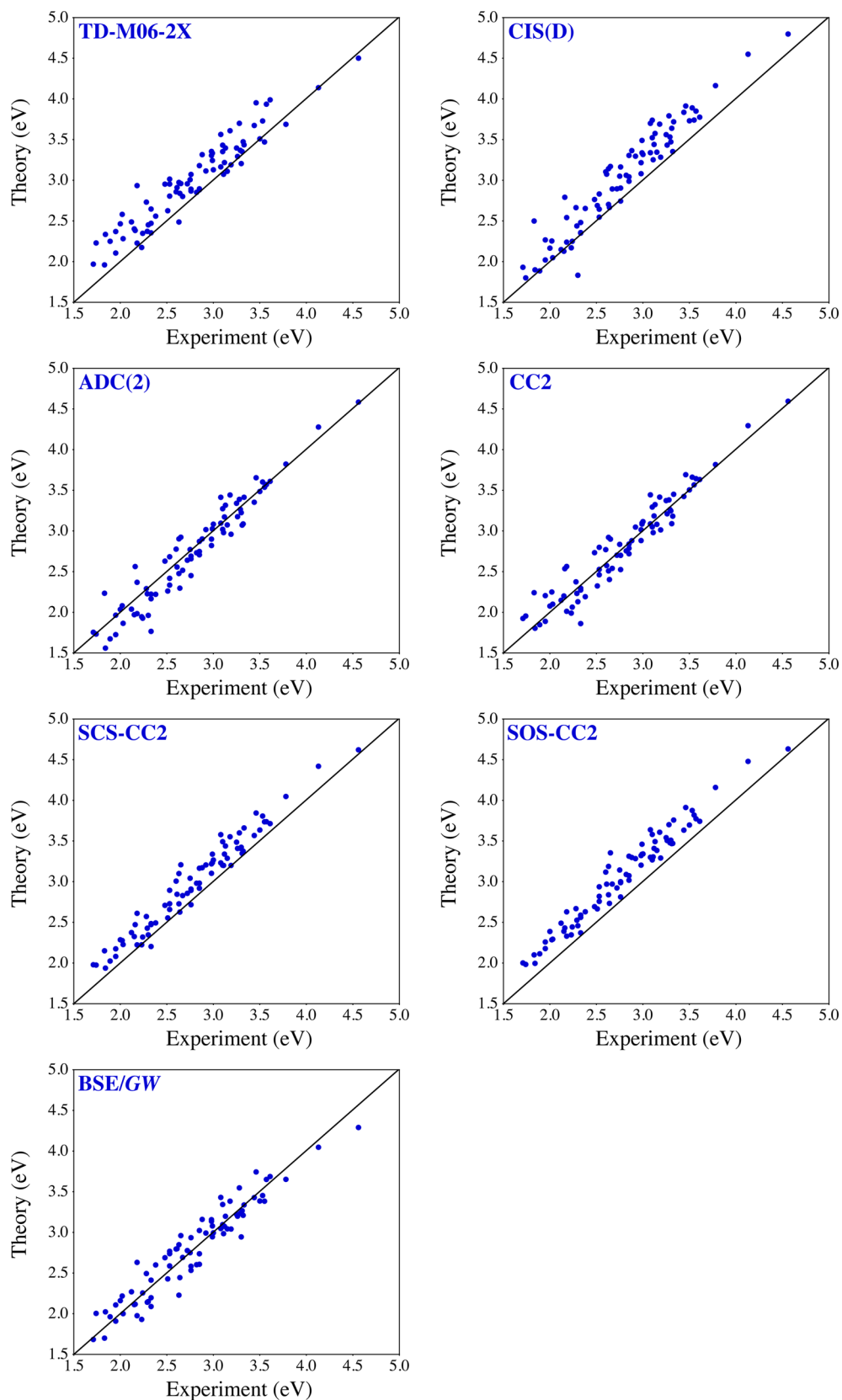
Figure 6. Correlation plots between the computed \Delta E^{0-0}(\text{cLR}, \text{eq}) and the experimental AFPC energies for all tested methods. All values are in eV. The central line indicates a perfect theory–experiment match. These graphs correspond to the default PCM parameters.
