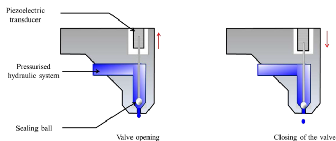
Figure 2. Diagram of operation of the generator opening valve.
