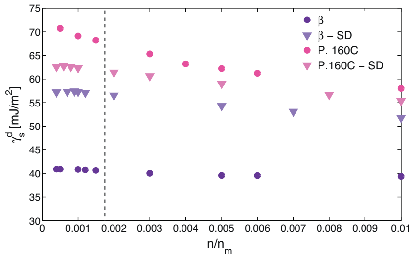
Fig. 8. Surface heterogeneity analysis of \beta mannitol samples, before and after spray drying.
