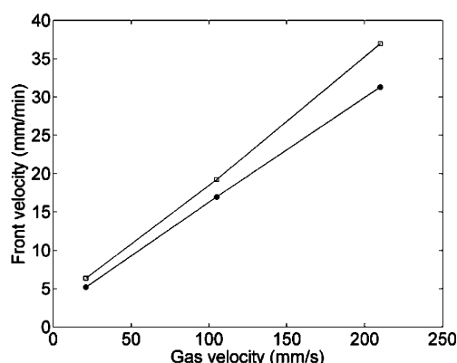
Figure 16. Experimental (●) and theoretical (□) chemical front velocity as a function of Darcy gas velocity.
