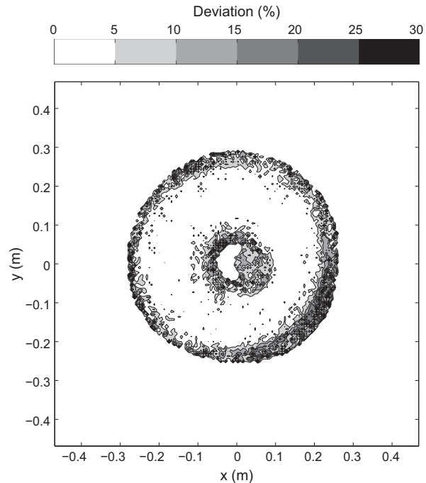
Fig. 9. Typical deviation between two runs 1 m away from the focal spot.
