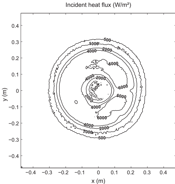
Fig. 3. Heat flux mapping 1 m away from the focal spot.
