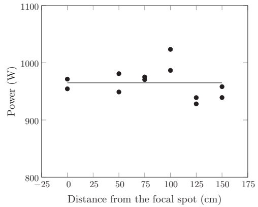
Fig. 8. Incident power for all runs. Dot individual value, continuous line average value.
