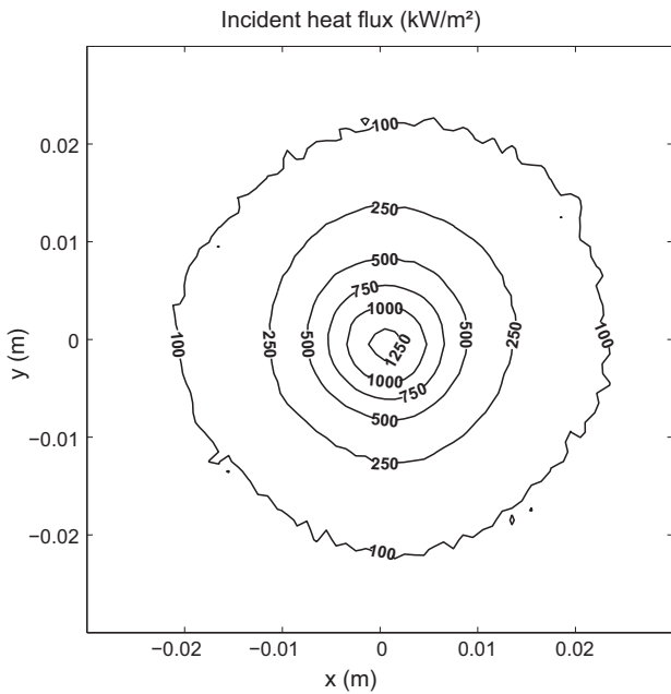
Fig. 6. Heat flux mapping at the focal spot.
