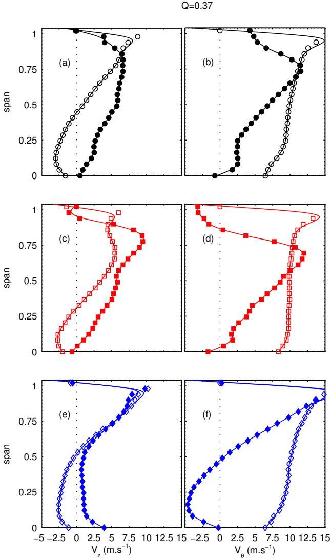
Figure 8: LDA measurements at Z_p = 5 mm downstream of the front rotor. Q_v = 0.37 m 3 .s -1 . (a-c-e): axial velocity V_z ; (b-d-f): tangential velocity V_\theta . (a-b): \circ —JW1 FR , \bullet —JW1. (c-d): \square —JW2 FR , \blacksquare —JW2, \diamond —JW3, \blacklozenge —JW3
