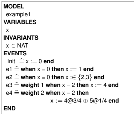
Figure 10: Partially mixed Event-B model and MDP semantics for Example 1
