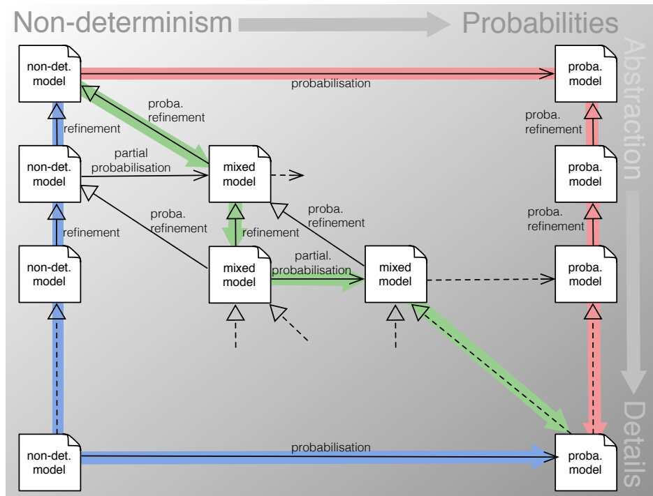
Figure 1: How to introduce probabilities within Event-B?
