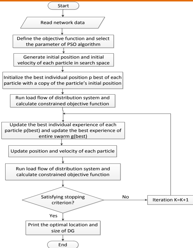
Fig. 4 Particle swarm optimization.
