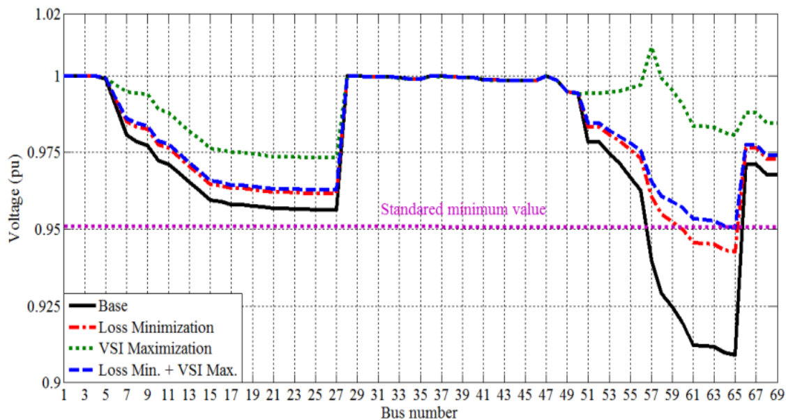
Fig. 10 Voltage profile before and after adding DG of type (4)
