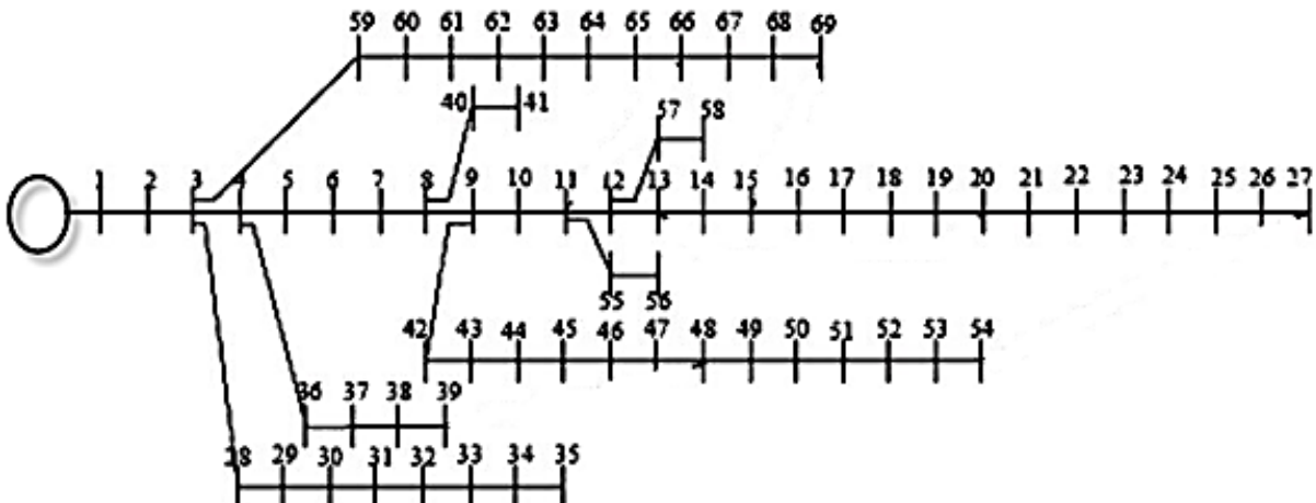
Fig. 6 Single line diagram of IEEE 69-bus system
