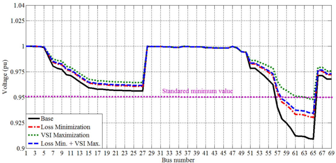
Fig. 8 Voltage profile before and after adding DG of type (2)
