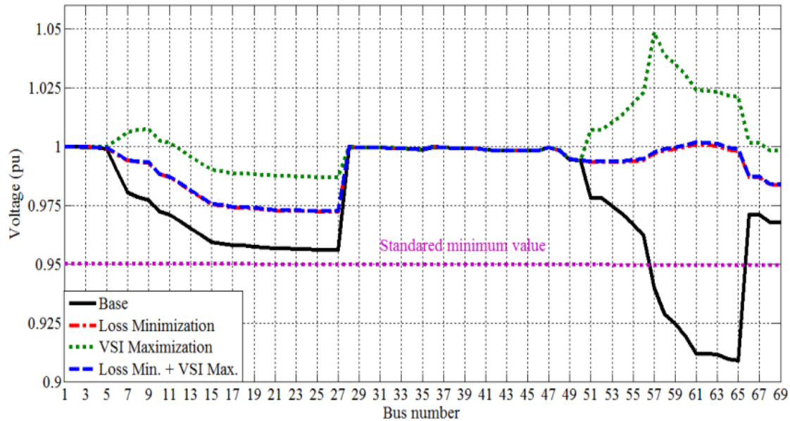
Fig. 9 Voltage profile before and after adding DG of type (3)
