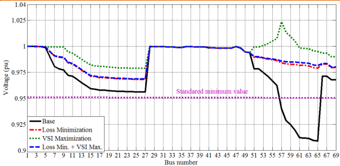
Fig. 7 Voltage profile before and after adding DG of type (1)
