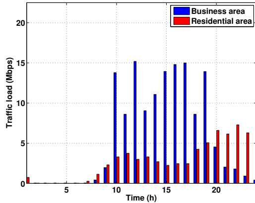
Fig. 2: Daily traffic load observed on business and residential area RRHs during a workday [1].
