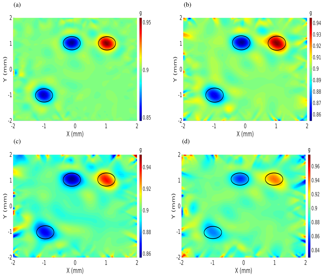
Figure 4: Reconstructions of the anisotropy factor g for four different noise levels \sigma_m on the synthetic data. The original phantom medium to reconstruct was shown in figure 1. (a) reconstructed g image with noiseless data (b) reconstructed g image, for \sigma_m = 3\% (c) reconstructed g image, for \sigma_m = 6\% (d) reconstructed g image, for \sigma_m = 10\% . The solid circles indicate the exact inclusion locations.
