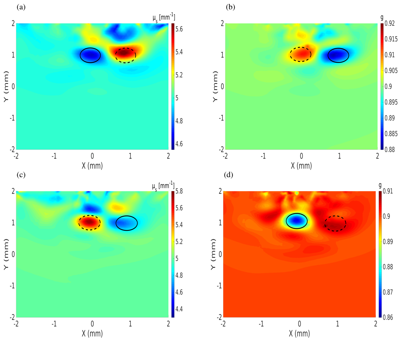
Figure 5: Simultaneous reconstructions of the scattering coefficient \mu_s and the anisotropy factor g . Left column : Reconstructed \mu_s images. Right column : Reconstructed g images. Top row : Test case 1, inclusion A in scattering coefficient and inclusion B in anisotropy factor. Bottom row : Test case 2, inclusion A in anisotropy factor while inclusion B in scattering coefficient. The solid circles indicate the exact positions while the dashed circles depict the crosstalk zones.
