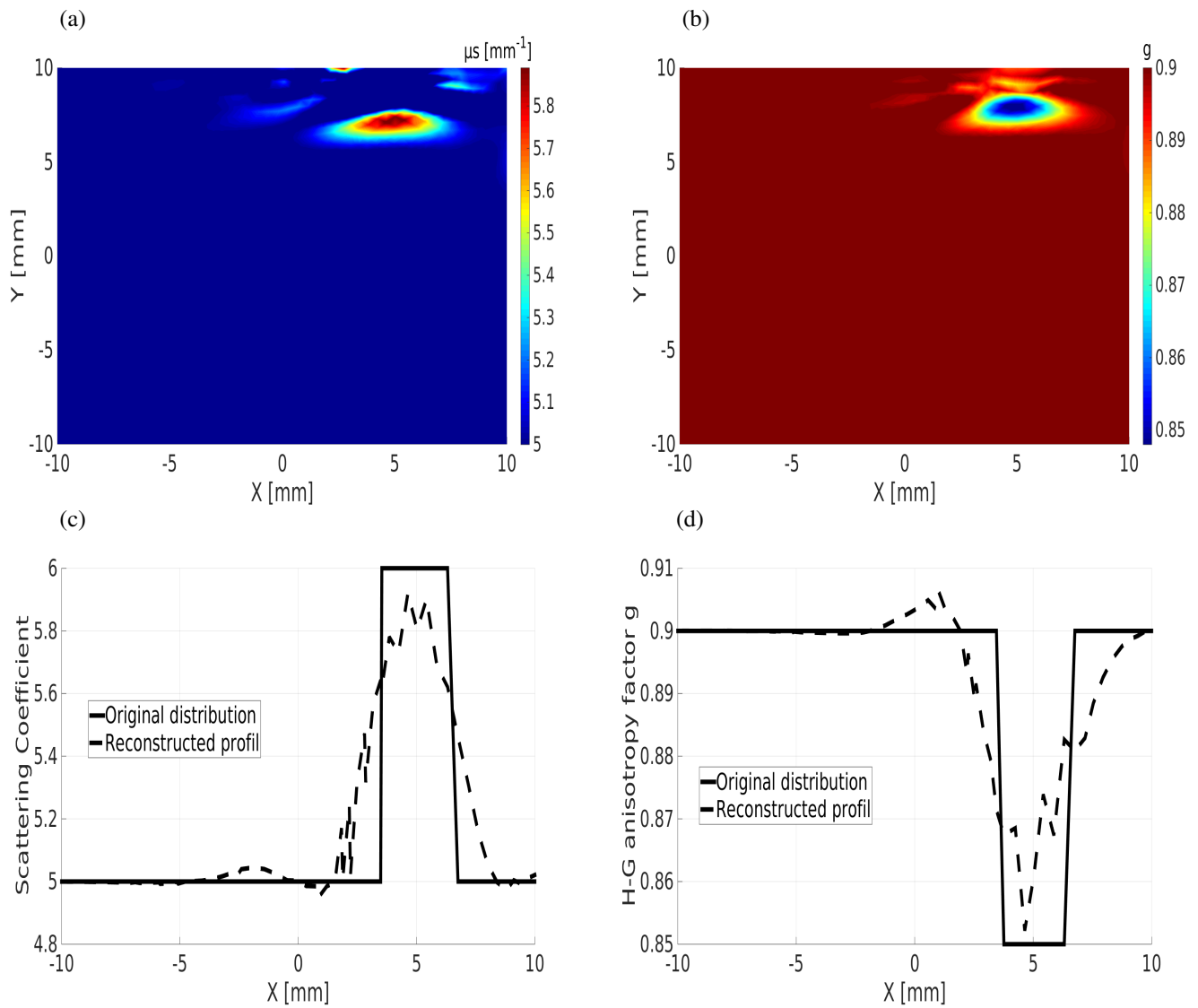
Figure 6: Simultaneous reconstructions of the scattering coefficient \mu_s and the anisotropy factor g for the 2 \text{ cm} \times 2 \text{ cm} domain. (a) : Reconstructed \mu_s image. (b) : Reconstructed g image. (c) : \mu_s Cross-section. (d) : g Cross-section. We started the minimization using the homogeneous background optical properties : \mu_a = 0.05 \text{ mm}^{-1} , \mu_s = 5 \text{ mm}^{-1} and g = 0.9 .
