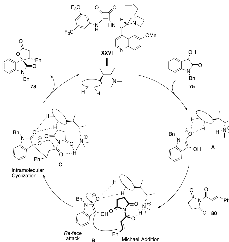
Scheme 24. Asymmetric cascade Michael/cyclization reaction performed on 3-hydroxyoxindoles/ N -acylated succinimides as donor/acceptor system. A–C are hypothesized intermediates on the catalytic cycle proposed.
