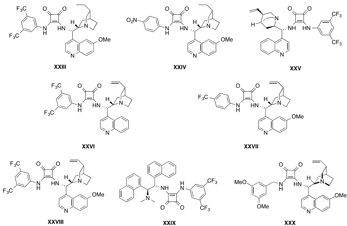
Figure 6. Squaramide based organocatalysts reported in the present section.
