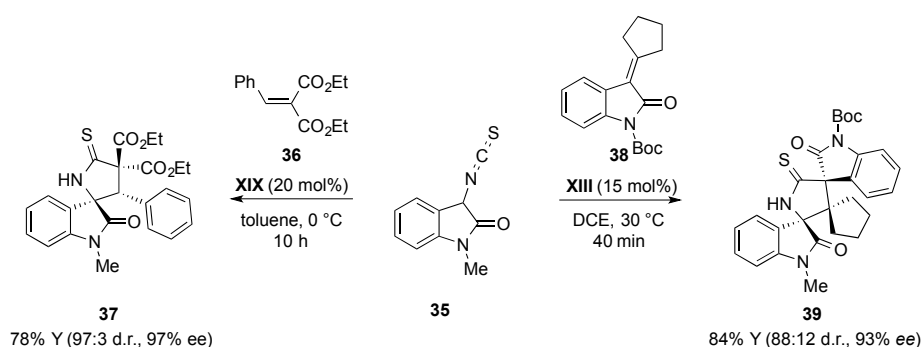
Scheme 9. 3-Isothiocyanate oxindoles as versatile substrates for the synthesis of densely functionalized spirooxindoles.
