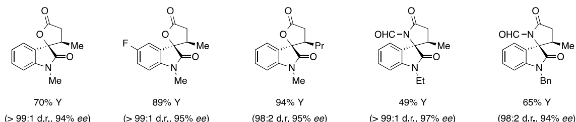
Scheme 23. Organocatalyzed Michael/cyclization cascade reaction for the construction of spirocyclic oxindole- \gamma -lactones/lactams.
