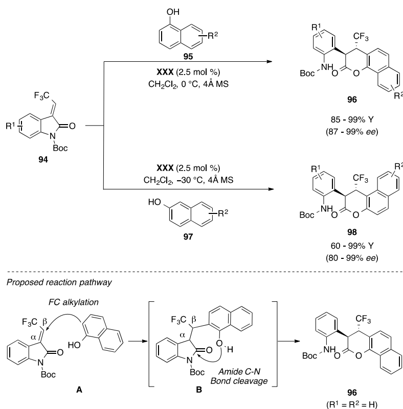
Scheme 28. Friedel-Crafts/lactonization domino reaction developed by Zhao and co-workers and suggested reaction pathway.
