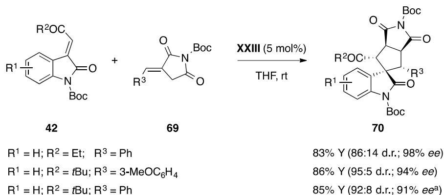
Scheme 21. Organocatalytic cascade Michael/Michael addition for spirooxindoles containing five contiguous stereocenter. a The reaction was carried out on gram scale.
