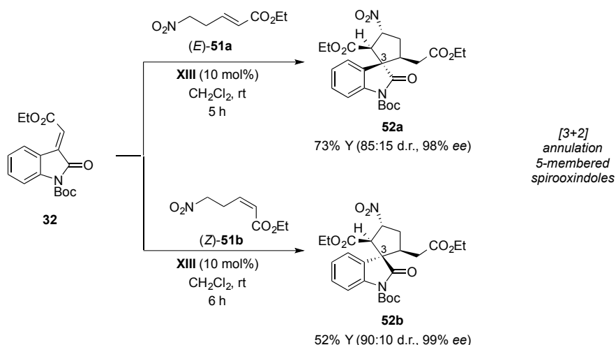
Scheme 14. Synthesis of \beta -nitro spirocyclopentane indolinones 52 via double Michael cascade in the presence of Takemoto's catalyst XIII .
