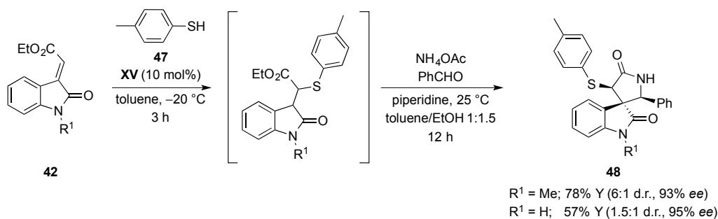
Scheme 12. Synthesis of spiro- \gamma -lactam oxindoles via cascade reaction catalyzed by catalyst XV .
