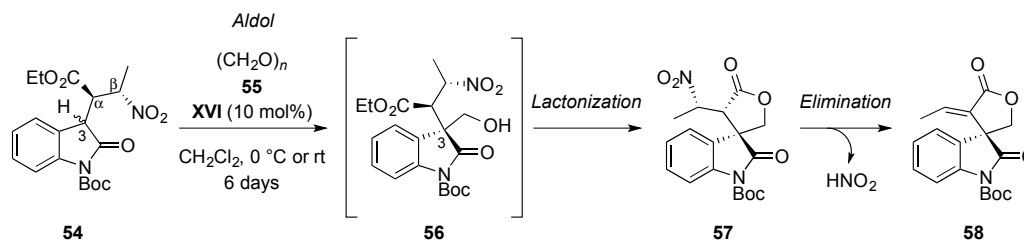
Scheme 16. Synthesis of 3-spiro- \alpha -alkylidene- \gamma -butyromactone oxindoles 58 in the presence of Cinchona-derived thiourea catalyst XVI .
