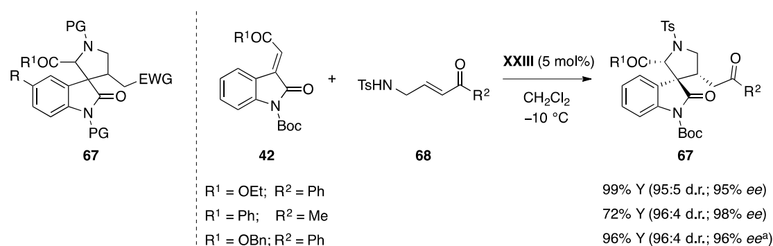
Scheme 19. Asymmetric cascade aza-Michael/Michael addition for spiro[pyrrolidine-3,3'-oxindoles]s 67 .
