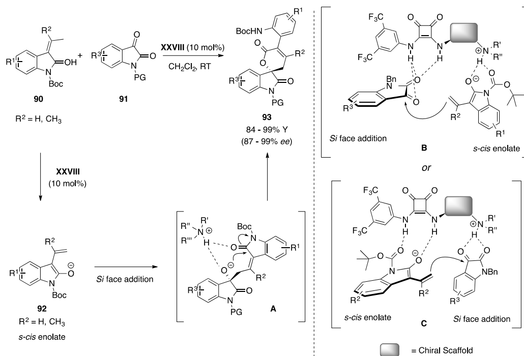
Scheme 27. Asymmetric aldol/lactonization sequence for the synthesis of spirooxindole dihydropyranones 93 . A is the hypothesized intermediate on the reaction pathway, while B and C are proposed alternative models for explaining the dual activation of nucleophile and electrophile.
