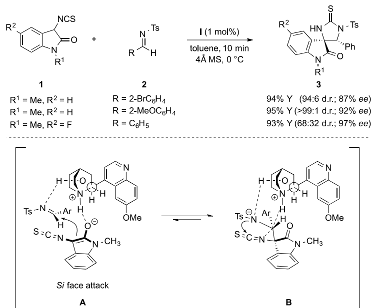
Scheme 1. Synthesis of spiro[imidazolidine-2-thione-4,3'-oxindole] via domino Mannich/Cyclization process and proposed transition states where A and B are the suggested intermediates (Y = Yield).
