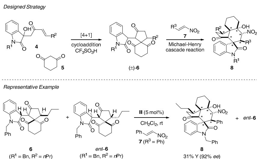
Scheme 2. Synthesis of spirooxindole polycycles bearing a spiro[4,5]decane system.
