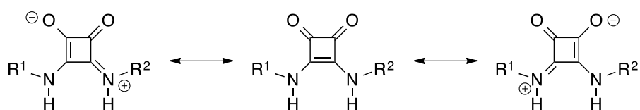
Figure 5. (a) H-Bond donor ability of squaramide and thiourea; (b) Lone pairs conjugation and resonance forms of the aromatic system.
