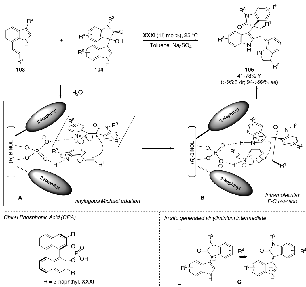
Scheme 30. (CPA)-catalyzed Michael addition/intramolecular Friedel-Crafts cascade reaction toward the construction of cyclopenta[ b ]indole and spirooxindole scaffold. A–C are postulated intermediates on the mechanism of the reaction.
