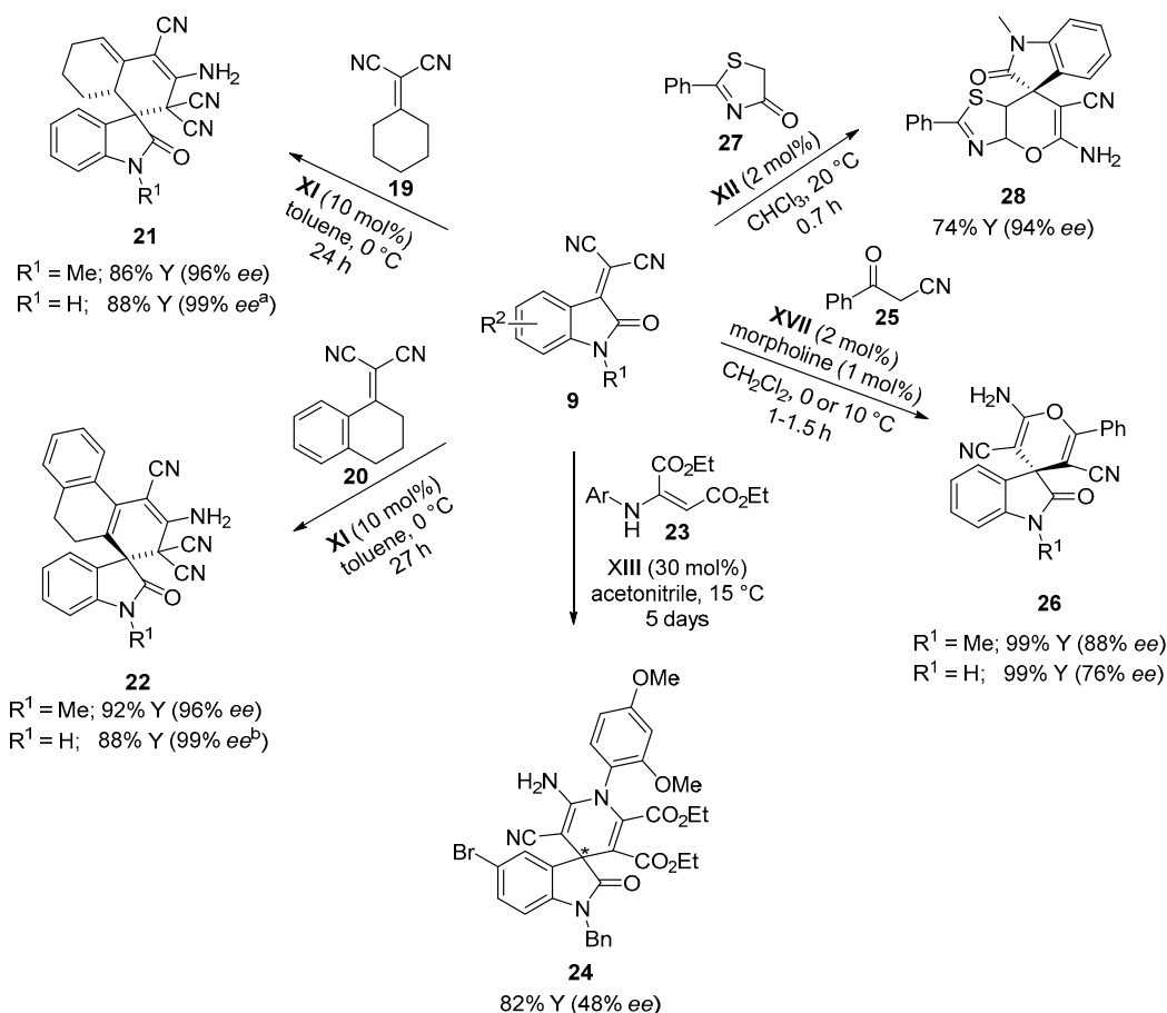
Scheme 6. Recent examples of spirooxindoles synthesized from isatylidene malonitrile derivatives 9 through cascade processes involving Michael addition/cyclization sequence. a Three-component reaction performed during 36 h. b Three-component reaction performed during 48 h.
