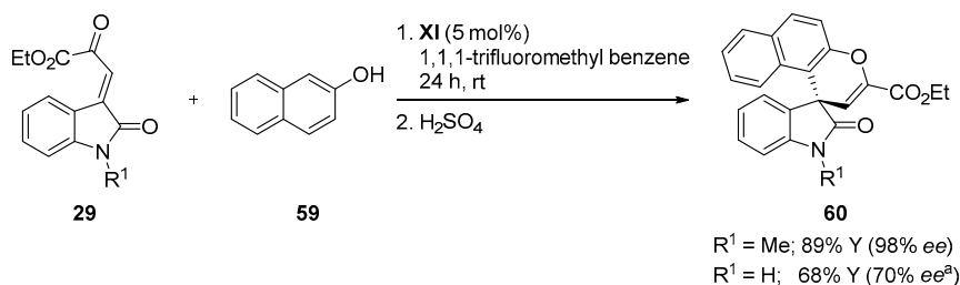
Scheme 17. Synthesis of spirooxindole-naphthopyrans 60 in the presence of catalyst XI . a 86% ee after recrystallization.
