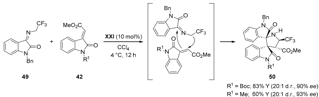
Scheme 13. Domino Michael-Mannich [3 + 2] cycloaddition for the asymmetric synthesis of 3,3'-pyrrolidinyl-dispirooxindoles 50 .
