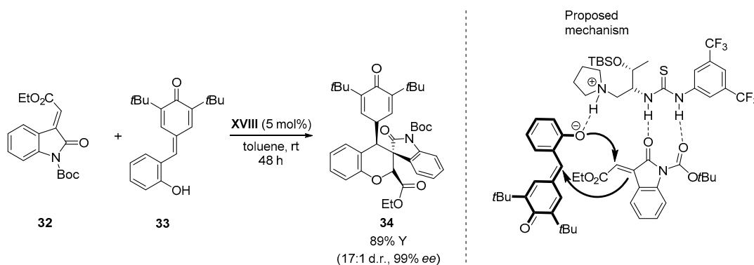
Scheme 8. Synthesis of chromans 34 with an oxindole moiety catalyzed by XVIII .
