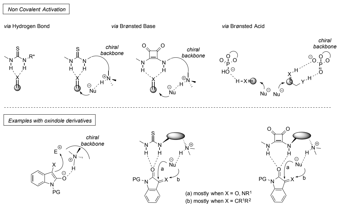
Figure 2. Examples of non-covalent interactions in a substrate/reagent/catalyst system.
