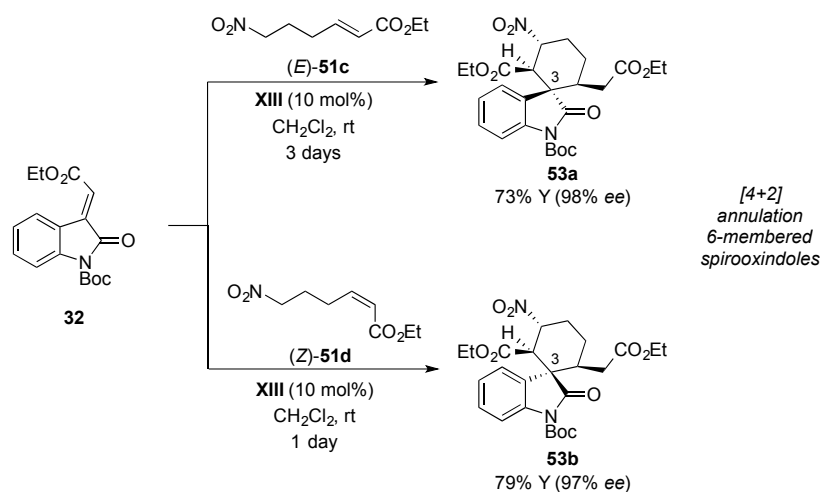
Scheme 15. Synthesis of \beta -nitro spirocyclohexane indolinones 53 via double Michael cascade in the presence of Takemoto's catalyst XIII .
