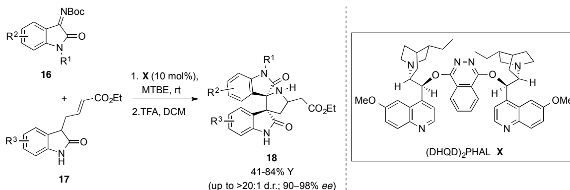
Scheme 5. Organocatalytic Mannich/Boc-deprotection/aza-Michael sequence developed by Enders and co-workers.
