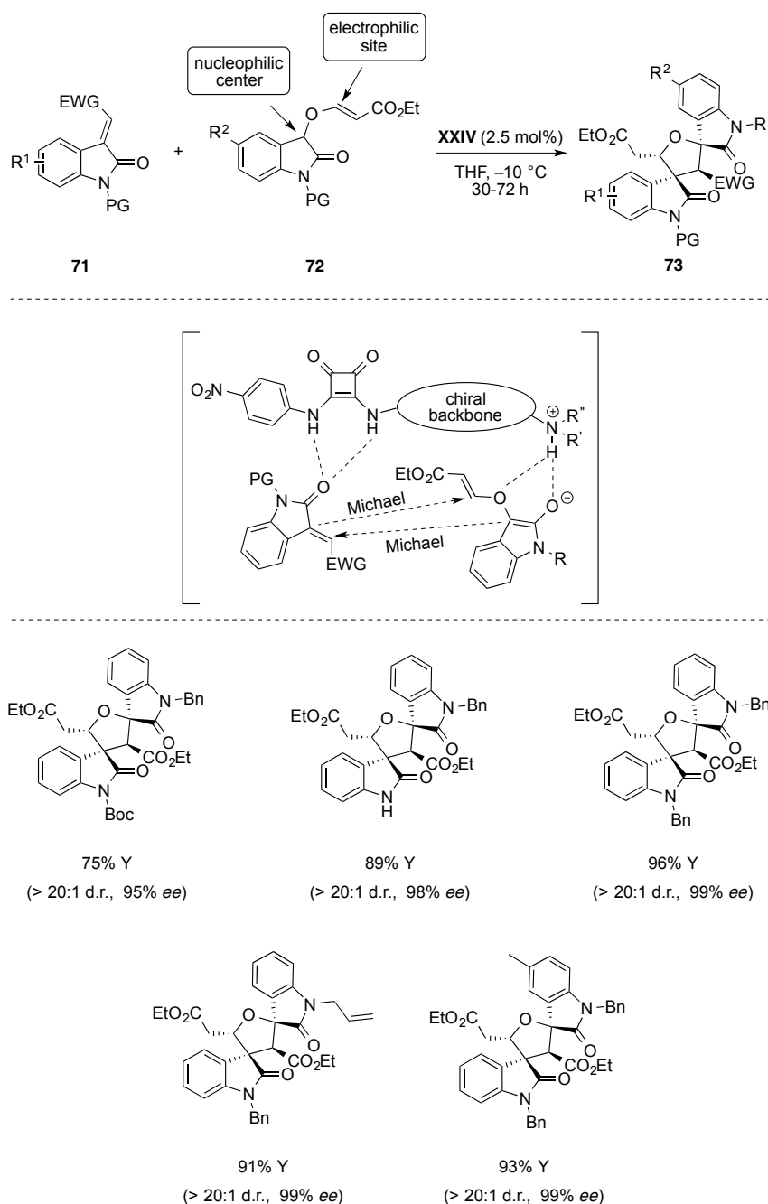
Scheme 22. Asymmetric enantioselective tandem Michael/Michael reaction to bispirooxindoles 73 .
