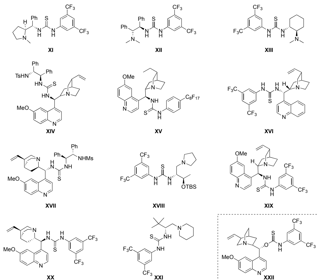
Figure 4. Thiourea and thiocarbamate organocatalysts used in this section.
