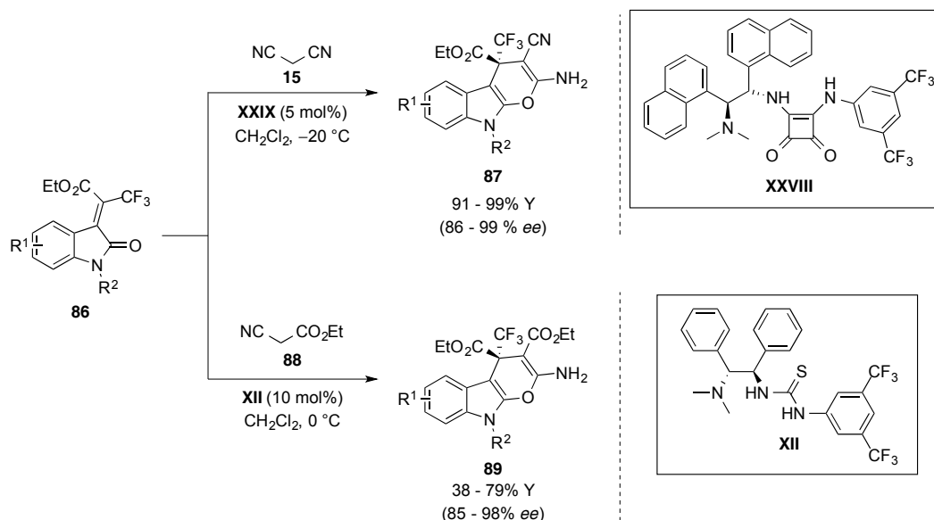
Scheme 26. Synthesis of dihydropyranoindole derivatives, a comparison between squaramide-based and thiourea catalyst.
