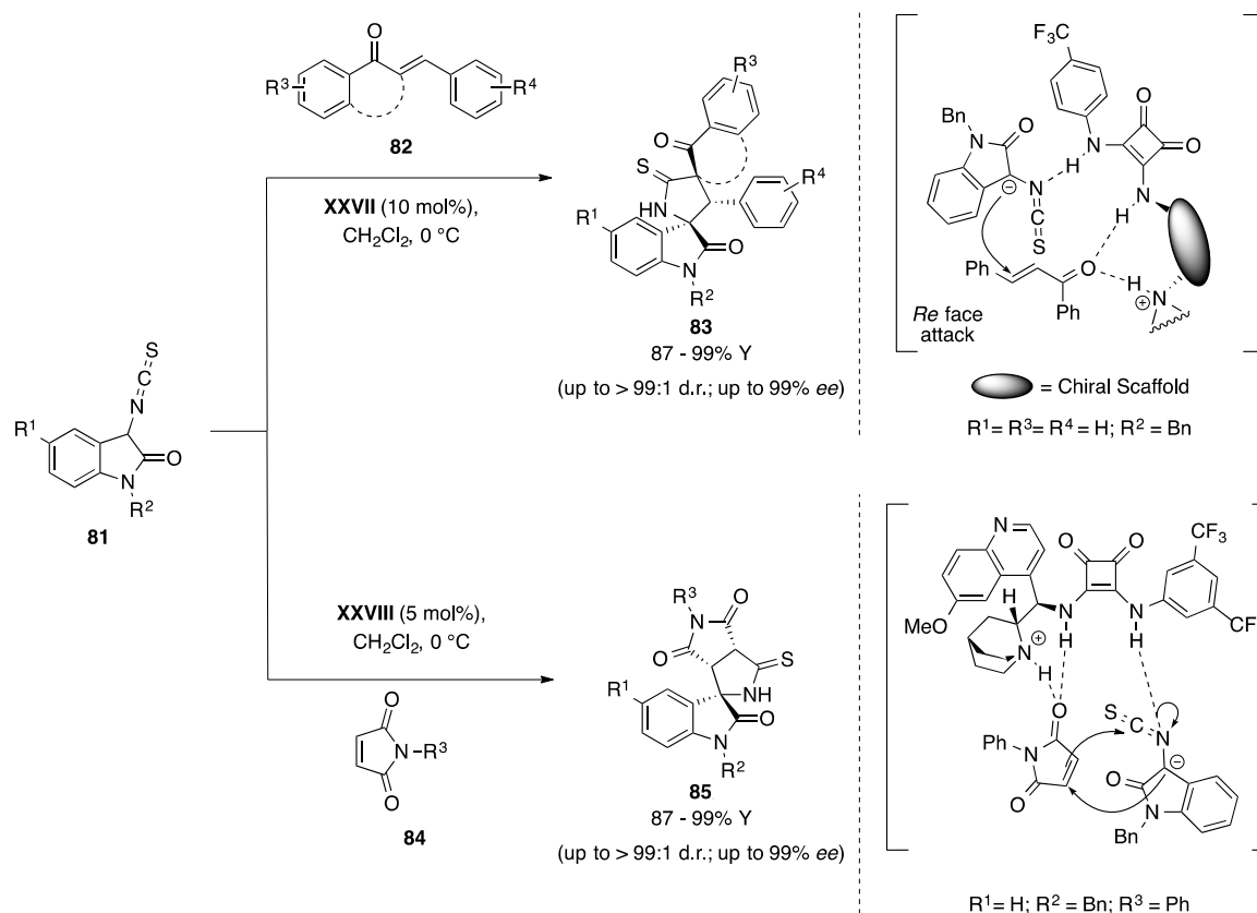
Scheme 25. Du's research toward the preparation of pyrrolidinyl spirooxindoles 83 and 85 employing respectively chalcones 82 and maleimides 84 .
