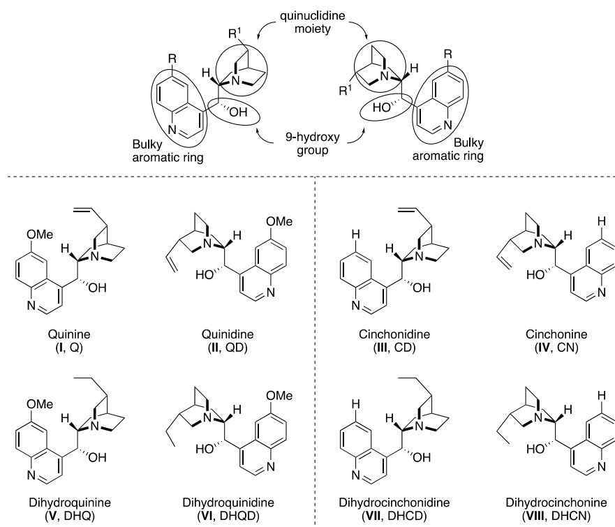
Figure 3. Representative examples of Cinchona alkaloids.
