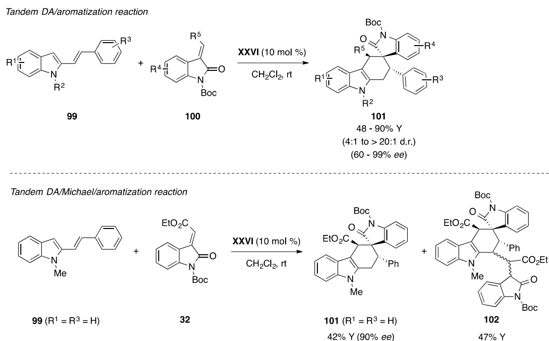
Scheme 29. Diels-Alder (DA)/aromatization sequence and triple DA/Michael/aromatization domino process.
