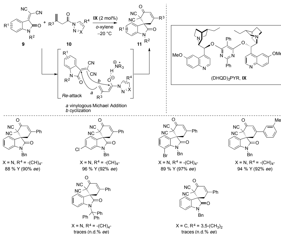
Scheme 3. Michael/cyclization cascade reaction to spirocyclic oxindoles catalyzed by (DHQD) 2 PYR ( IX ).
