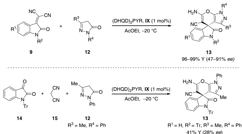
Scheme 4. Michael/cyclization cascade reaction catalysed by (\text{DHQD})_2\text{Pyr} ( IX ) when pyrazolone 12 was employed as Michael donor.
