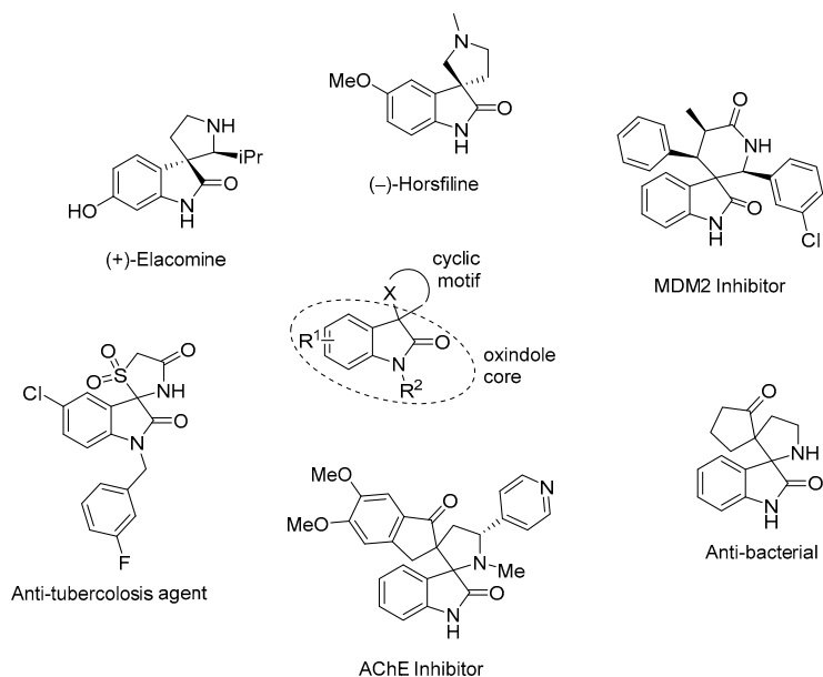
Figure 1. Examples of bioactive compounds built around the oxindole framework.
