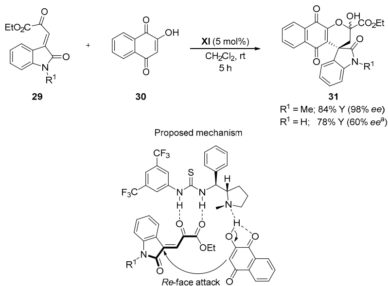
Scheme 7. Synthesis of hybrid spirooxindole-naphthoquinones through catalysis with proline-based catalyst XI . a Reaction was carried out at 5 °C.
