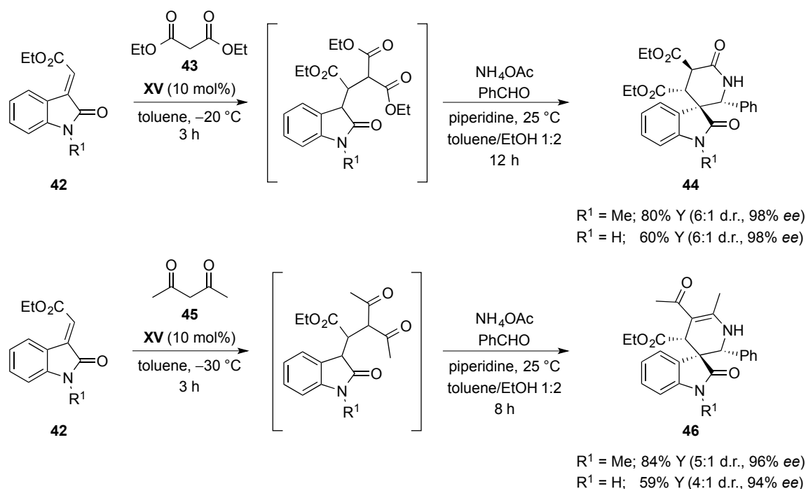
Scheme 11. Synthesis of piperidone and tetrahydropyridine rings bearing spirooxindoles in the presence of recyclable catalyst XV .
