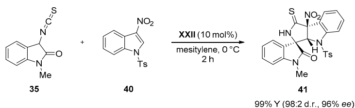
Scheme 10. Asymmetric synthesis of polycyclic spirooxindoles in the presence of amino-thiocarbamate catalyst XXII .
