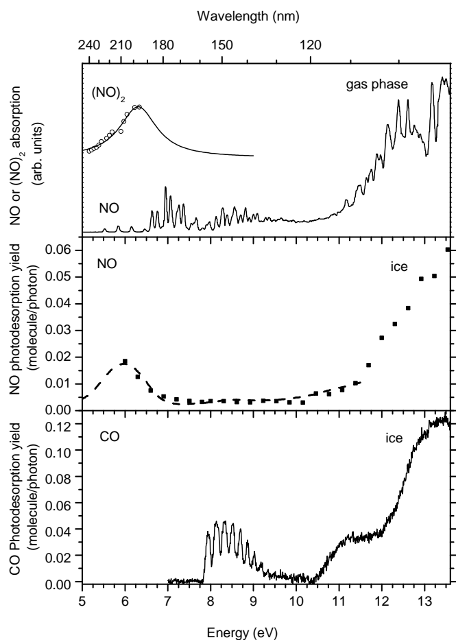
Fig. 1. Upper panel: Electronic spectrum of gas-phase NO from Chang et al. (1993) and electronic spectrum of gas-phase (NO) 2 from Forte & Van Den Bergh (1978) (open dots) and its Lorentzian fit (solid line). Middle panel: NO photodesorption spectrum of 10 ML thick NO ice on HOPG at 10 K between 6 and 13.6 eV (filled squares). Large energy steps of 0.3 eV were used to avoid ice ageing. Absorption spectrum of pure solid NO from Lu et al. (2008) between 5 and 11.7 eV (dashed line). The absorption spectrum is scaled to the photodesorption spectrum. Lower panel: CO photodesorption spectrum of a 20 ML thick CO ice on gold at 10 K between 7 and 13.6 eV (Dupuy et al. 2017)
