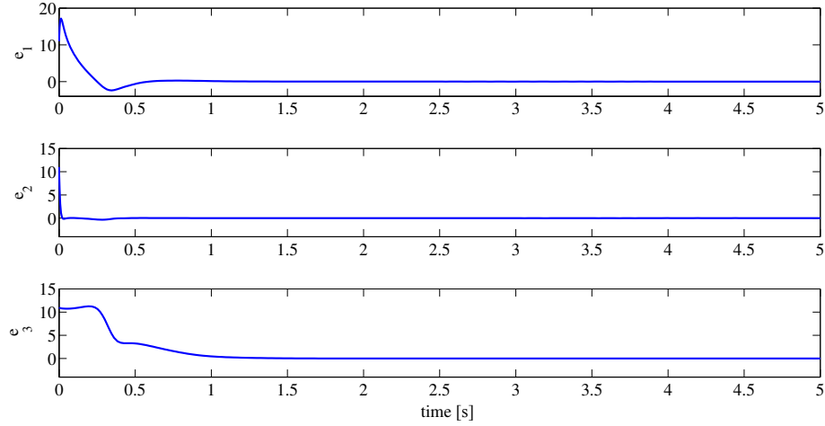
Figure 2: State estimation errors
