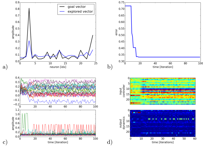
Fig. 2. Explored dynamics toward a goal. (a) ANN makes to converge the RNN neurons (in blue) to some desired dynamics (in black) thanks to prediction error. (b) the ANN prediction error diminishes to reach a local minimal value during the first 20 iterations. (c-d) Dynamics of the ANN to control the dynamics of the RNN.
