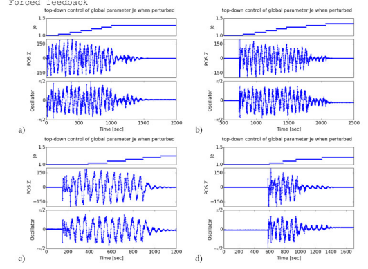
Figure 3: Feedback control of the global parameter J_e . When a strong perturbation is imposed on the structure, an oscillatory regime is established by the top-down controller to absorb the shock with a high amplitude till their attenuation.
