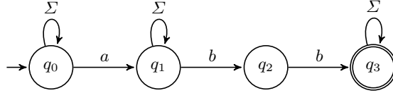
Fig. 5: Automaton A_2 defining the Boolean query \mathbf{Q}_2 with alphabet \Sigma = \{a, b, c\}
