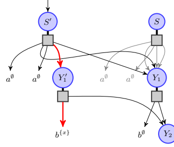
Fig. 8: G' on \Sigma^{\mathcal{V}} with \text{pat}(G') = \text{pat}(G)*[x/5] .
