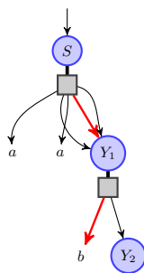
Fig. 5. G with red thick path to the shared position 5.
