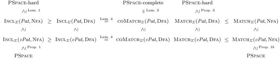
Fig. 4. PTIME reductions for regular inclusion and matching problems.
