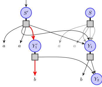
Fig. 6. Partially uncompressing G at position 5.
