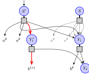
Fig. 7. G' on \Sigma^V with pat(G') = pat(G) * [x/5] .
