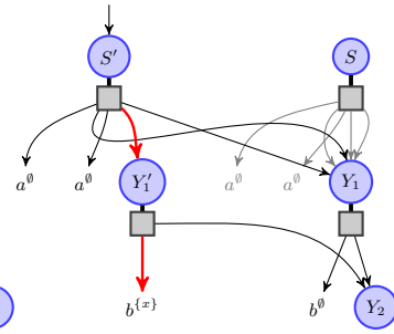
Fig. 7. G' on \Sigma^{\mathcal{V}} with pat(G') = pat(G)*[x/5] .
