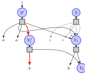
Fig. 6. Partially uncompressing G at position 5.
