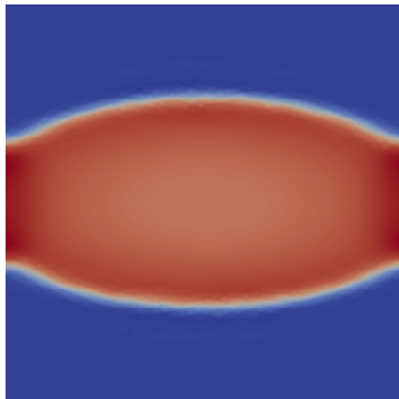
Figure 6: Reference solution for the transmembrane potential at time T = 16\text{ms} for the BR model in 2D plotted as a function of x \in [0, 1] \times [0, 1] .
