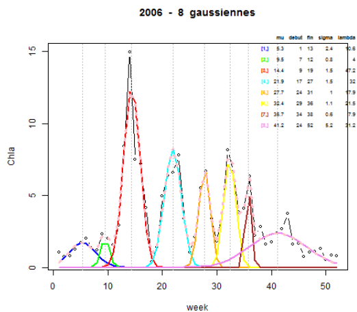
Fig. 6. 8 Estimated Gauss Curves from the Chla 2006-subsequence in the southern bight of the North Sea. Chla unit is in \mu\text{g}\cdot\text{l}^{-1} .
