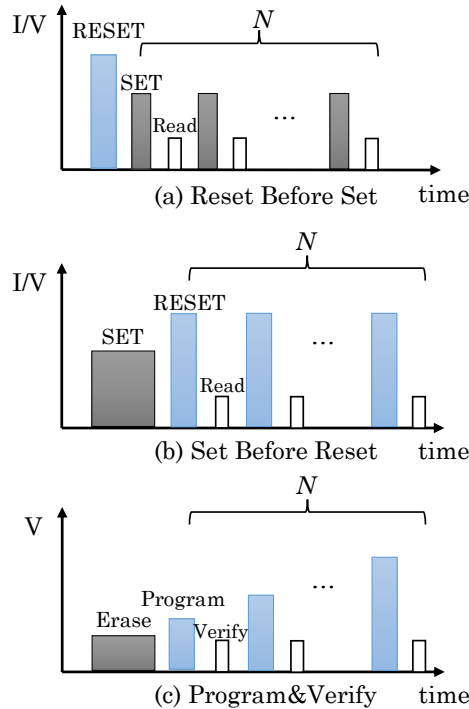
Fig. 6. MLC write model ((a,b) apply to MLC PCM and MLC ReRAM, whereas (c) applies to MLC Flash) [16].
