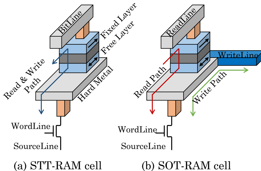
Fig. 4. Comparison of the STT-RAM and SOT-RAM cell model.
