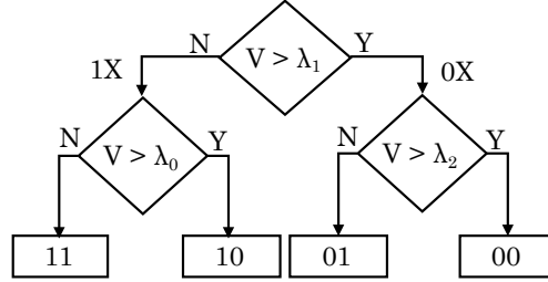
Fig. 5. MLC read model. Note that \lambda_0 < \lambda_1 < \lambda_2 .
