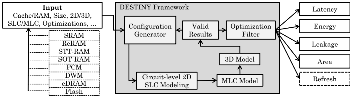
Fig. 2. High-level overview of the DESTINY framework.
