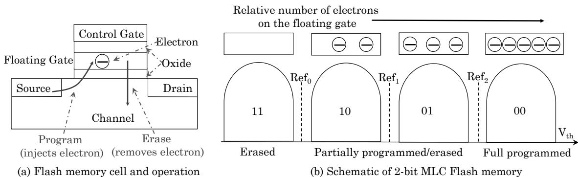
Fig. 1. An illustration of Flash memory.
