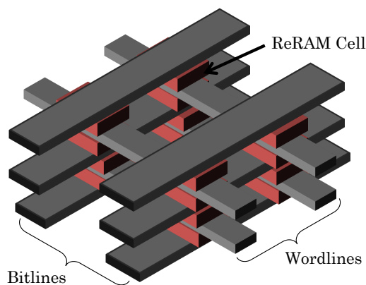
Fig. 7. Four-layer monolithically stacked ReRAM. Storage elements are sandwiched directly between layers of wordlines (south-east orientation) and bitlines (south-west orientation).
