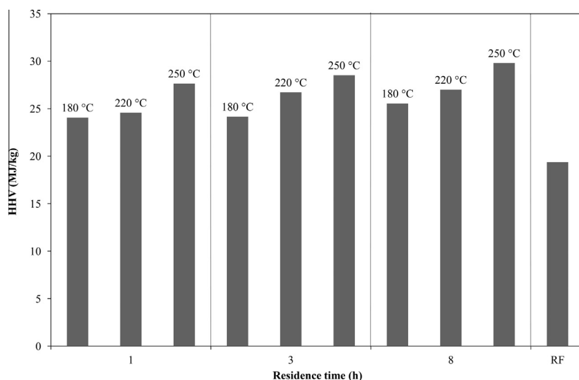
Fig. 5. HHVs at different temperatures and residence times.
