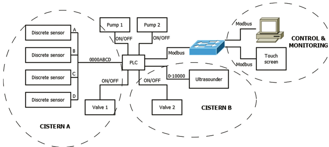
Fig. 2. Training platform network.
