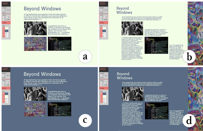
Figure 7. Contextify accepts inputs for tailoring layout under four reading conditions: day (a-b) vs. night (c-d); preview (a-c) vs. full detail (b-d).
