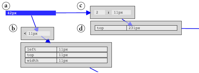
Figure 9. StyleBlocks supports arbitrary values (a), operators (limits (b) and ratios (c)) as well as CSS declarations (d).
