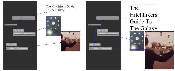
Figure 10. StyleBlocks : Designers create substrates that link the CSS properties of a web page. Here, a substrate generates the layout from a single value, 42 for the left page and 80 for the right one.
