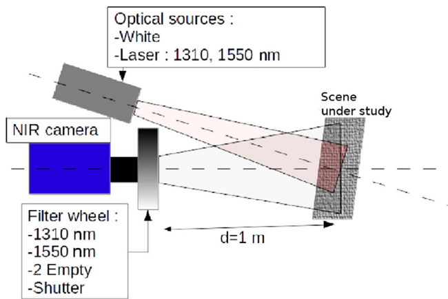
Fig. 3. Schematic top view of the apparatus.
