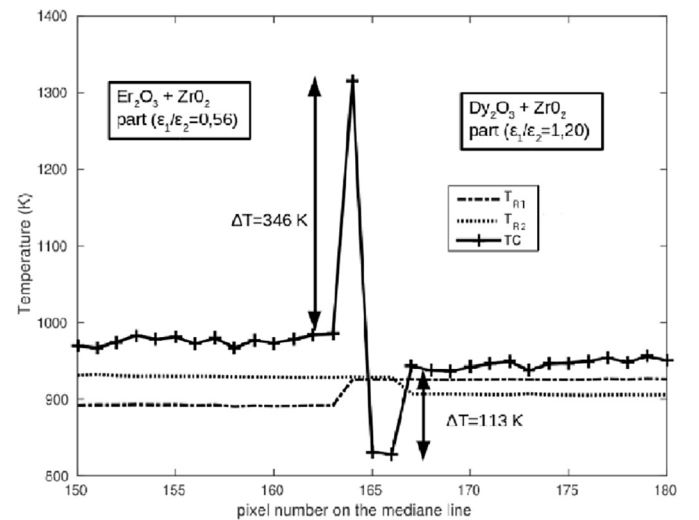
Fig. 2. Radiance and colour temperature on a profile of the “two-emissivity sample”.
