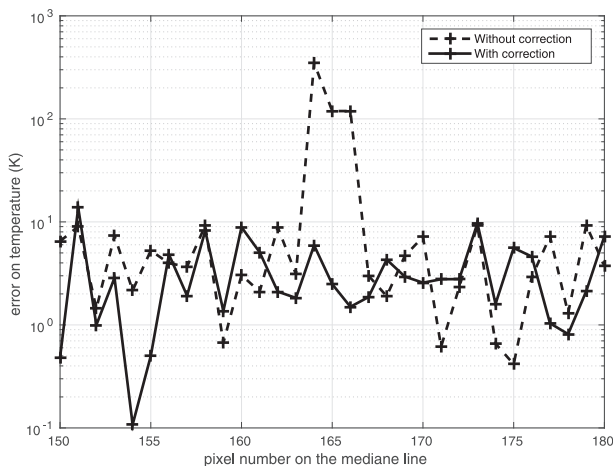
Fig. 5. Semi-log graph of the absolute temperature error before and after correction versus the pixel number.
