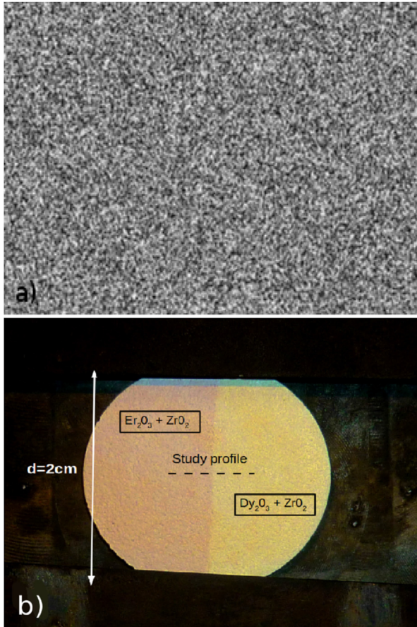
Fig. 1. Photograph of the scenes under study: a) Reference pattern (Perlin noise) for the distortion calculation by DIC; b) “Two-emissivity” sample for the temperature error evaluation (and the profile under study).
