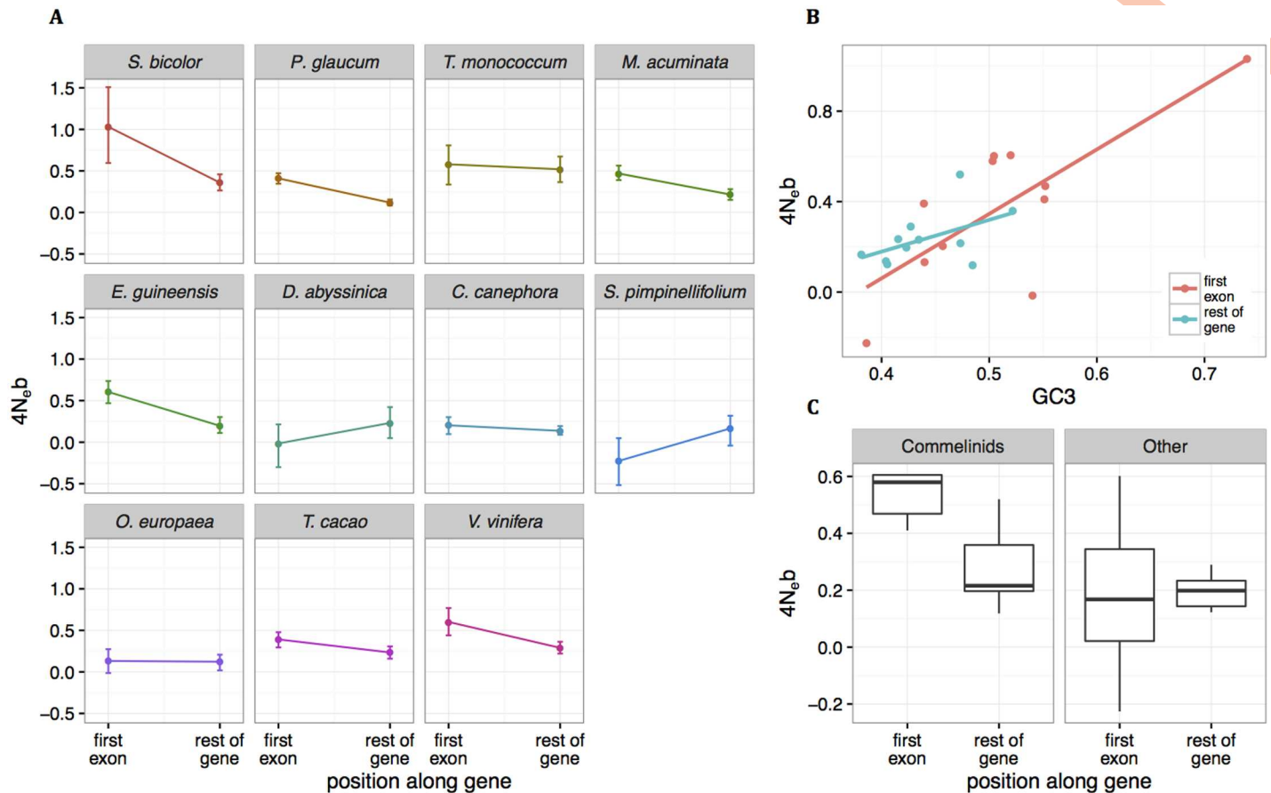
Fig 7. GC3 and gBGC gradients along genes. A: gBGC strength estimations ( 4N_{e}b ) for first exons (252 first bp of contigs) and rest of gene. Error bars indicate the 95% confidence intervals. With the exception of D. abyssinica and S. pimpinellifolium , all species exhibit stronger gBGC in the first exons compared to the rest of genes. B: Correlations between GC3 and gBGC strength in first exons (red) and rest of genes (blue). Each dot corresponds to one species. GC3 and 4N_{e}b tend to be positively correlated in both regions: \rho_{\text{Spearman}} = 0.591 , p-value = 0.061 for first exons and \rho_{\text{Spearman}} = 0.382 , p-value = 0.248 for the rest of genes. C: Comparison of 4N_{e}b estimates between first exons and rest of genes for Commelinids (all Monocots with the exception of D. abyssinica , left panel) and other species (right panel). 4N_{e}b values are higher in first exons compared to rest of genes in Commelinids species, while other species exhibit no differences between first exons and rest of genes.
