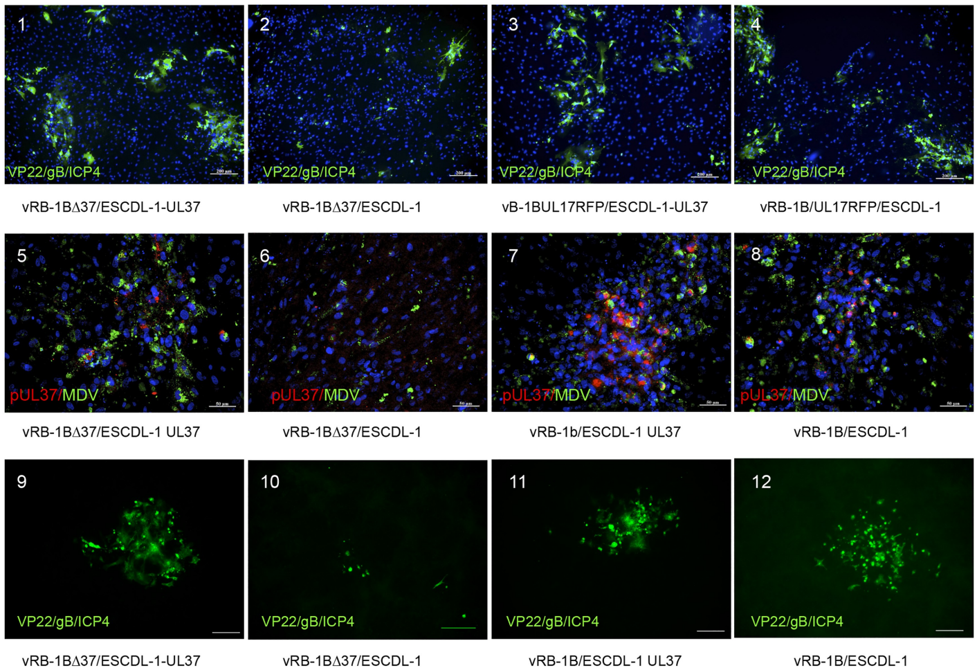
Fig 8. Expression of pUL37 in ESCDL-1 complements the deletion of UL37 ORF in BACRB-1B. Upper panel (1–4): Transfection of BACRB-1B \Delta 37 yields viral plaques on complementing cells: viral plaques were detected in ESCDL-1-UL37 by staining with Mabs B17 (anti-VP22), K11 (anti-gB) and E21 (anti-ICP4) and an Alexa Fluor ® 488 GAM conjugate (1). In ESCDL-1, BACRB-1B \Delta 37 did not yield a virus that could disseminate and only isolated positive cells could be seen (2). As a control, BACRB-1BUL17mRFP was transfected in either complementing or non-complementing parental cells, producing viral plaques on both (3 & 4). Scale bar = 200 \mu m. Middle Panel (5 to 8): vBACRB-1B \Delta 37 can be serially passaged in complementing cells and virus multiplication induces pUL37 expression in the ESCDL-1-UL37: BACRB-1B \Delta 37 (5,6) or BAC RB-1B (7,8) were transfected either in ESCDL-1-UL37 complementing cells or in ESCDL-1 and passaged once in the same cells. The development of viral infection by passage 2 of the vBACRB-1B \Delta 37 virus is seen in complementing cells (green fluorescence in 5) and coincides with the expression of pUL37 in infected cells (red fluorescence in 5); in non-complementing cells the same virus passage does not replicate (6). The parental virus (vBACRB-1B) transfected and passaged in the same conditions replicated equally well on ESCDL-1 and on ESCDL-1-UL37 (7 & 8). Scale bar = 50 \mu m. Lower Panel (9 to 12): vBACRB-1B \Delta 37 may be passaged at least 3 times in complementing cells and does not revert to a replicating virus when plated on non-complementing cells. The 3rd passage of vBACRB-1B \Delta 37 yielded typical viral plaques in complementing cells (9) whereas the same virus did not form plaques in ESCDL-1 (10). Again vRB-1B at the same passage developed equally well in both cells (staining as in the upper panel, except for HOECHST 33342). Scale bar = 200 \mu m.
