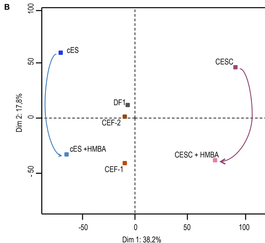
Fig 2. The HMBA treatment modifies the transcriptomic profile of both CESC and cES cells. (A) The Venn diagram illustrates the genes that are differentially expressed between CESC and cES cells treated with or without HMBA and uninfected or infected with vBAC20UL49GFP inoculums. (B) A PCA analysis was performed on the common genes identified from this study and those provided by the datasets GSE61221 for the CEF-1, GSE38168 for the CEF-2 and GSE47191 for the DF1 cells.
