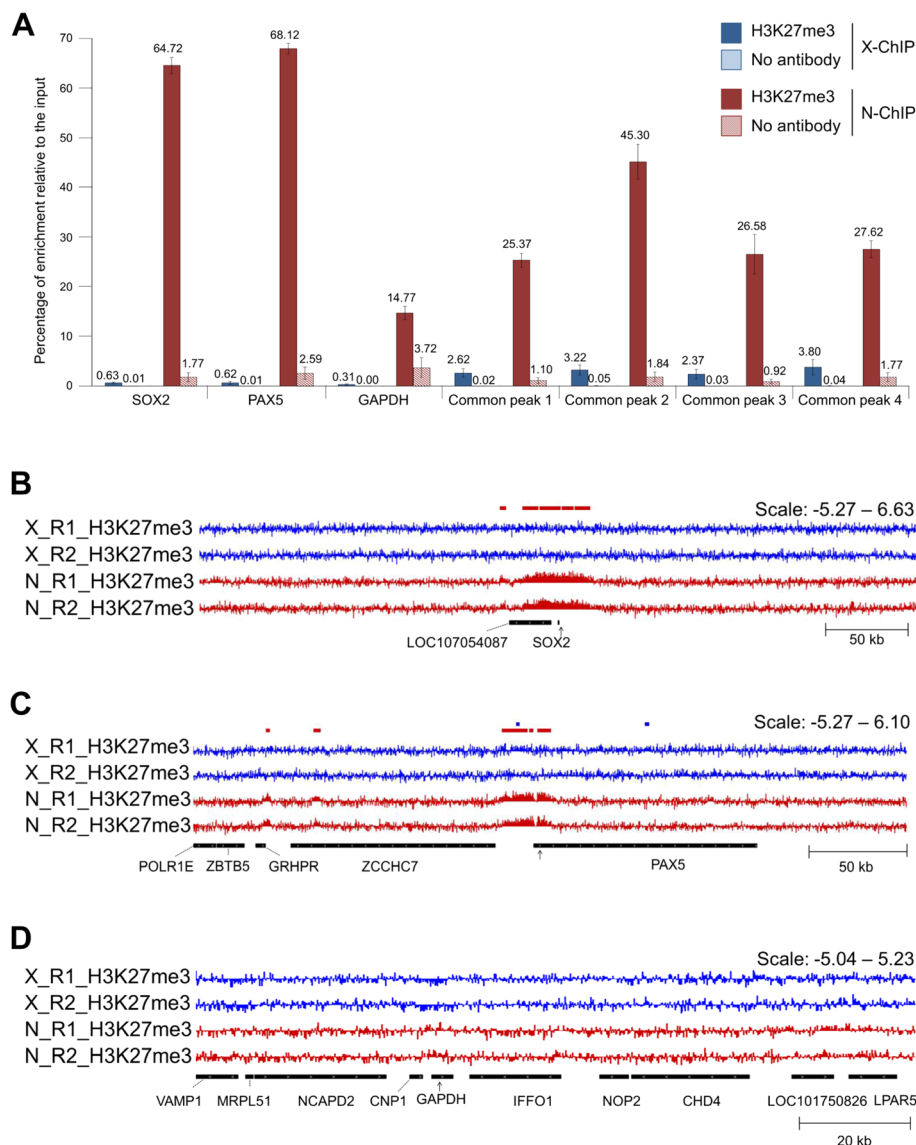
Fig. 2 N-ChIP and X-ChIP results at control loci. a Enrichment of H3K27me3 and no antibody relative to the input measured by qPCR at three control gene loci: SOX2 (chr9: 16,918,111–16,919,468), PAX5 (chrZ: 81,789,479–81,896,738) and GAPDH (chr1: 76,950,864–76,956,805), and at the localization of common enrichment detected with epic (see Fig. 1 legend for peak description). H3K27me3 enrichments are represented in blue for X-ChIP and in red for N-ChIP, no-antibody enrichments are represented in light blue for X-ChIP and in light red for N-ChIP. Error bars: SEM. b-d Visualization with IGV of H3K27me3 enrichment normalized to input [ \log_2(\text{IP}/\text{input}) ]. X-ChIP-seq muscle tracks are shown in blue, N-ChIP muscle tracks are shown in red. The colored boxes above the tracks represent broad peaks detected by epic in either X-ChIP-seq (blue) or N-ChIP muscle (red) replicates. The black arrows under the tracks represent the position of qPCR primers at (b) SOX2 , (c) PAX5 and (d) GAPDH
