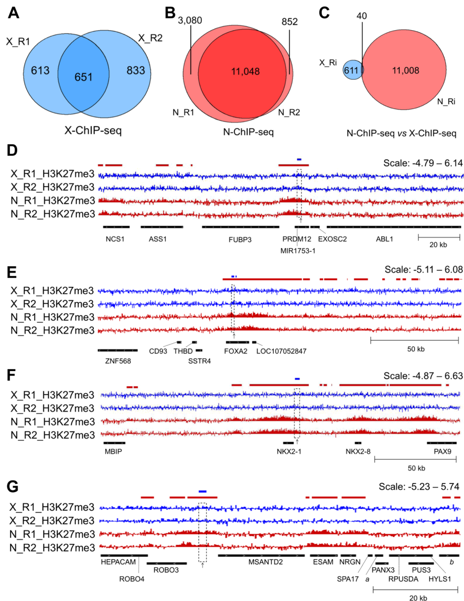
Fig. 1 N-ChIP-seq and X-ChIP-seq results. a–c Venn diagrams representing the overlap determined by intersectBed between H3K27me3 broad peak regions detected by epic. a X-ChIP-seq replicates. b N-ChIP-seq replicates. c Intersection between X-ChIP-seq and N-ChIP-seq peaks (only common peaks for each condition were considered). d–g Visualization with IGV of H3K27me3 enrichment normalized to input [ \log_2(\text{IP}/\text{input}) ]. X-ChIP-seq muscle tracks are shown in blue and N-ChIP-seq muscle tracks in red. The colored boxes above the tracks represent broad peaks detected by epic in either X-ChIP-seq (blue) or N-ChIP-seq muscle (red) replicates. The dashed boxes across the tracks represent the localization of a common peak (between methods). The black arrows under the tracks represent the position of qPCR primers used for Fig. 2A. d Common peak 1 (chr17: 6,422,600–6,424,599); e common peak 2 (chr3: 3,359,200–3,360,599); f Common peak 3 (chr5: 36,681,000–36,683,799); g common peak 4 (chr24: 262,600–264,199), a : LOC107055042, b : LOC101748751
