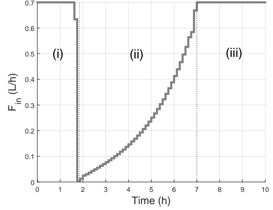
Fig. 1. Time evolution of the optimal influent flow rate
