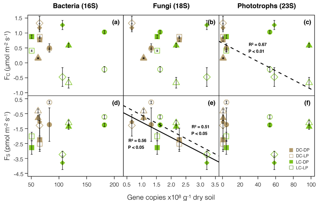
Fig. 5. Relationship between the net soil \text{CO}_2 and OCS fluxes for four soils (LB: squares, LG: circles, DBZ: triangles, TL: diamonds) as a function of the number of gene copies per gram of dry soil for bacteria (16S), fungi (18S) and phototrophs (23S) measured in the light (LP) and the dark (DP) after incubation for ~40 days in the light (LC) or the dark (DC). Significant linear model results are also displayed (solid lines for dark periods and dashed lines for light periods).
