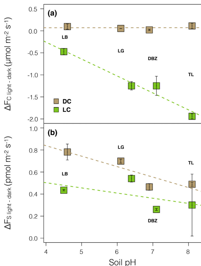
Fig. 4. Mean differences ( \pm SD, n = 3 ) in the net soil (a) \text{CO}_2 and (b) OCS fluxes measured during the light (LP) and the dark (DP) period for four soils of different pH incubated in the light (LC) or the dark (DC) for ~40 days.
