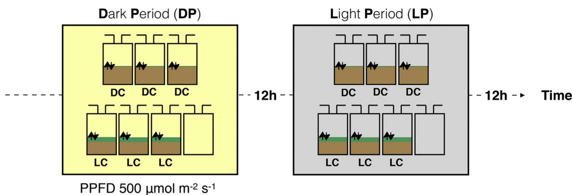
Fig. 1. Diagram illustrating the two-incubation treatments (applied from day 1 to day 40) and the two measurement treatments applied during the following 24 h of gas exchange measurements of the six microcosms from a given soil. DC: Dark Conditioning, LC: light conditioning, DP: dark period, LP: light period, WHC: water holding capacity, PPFD: photosynthetic photon flux density.
