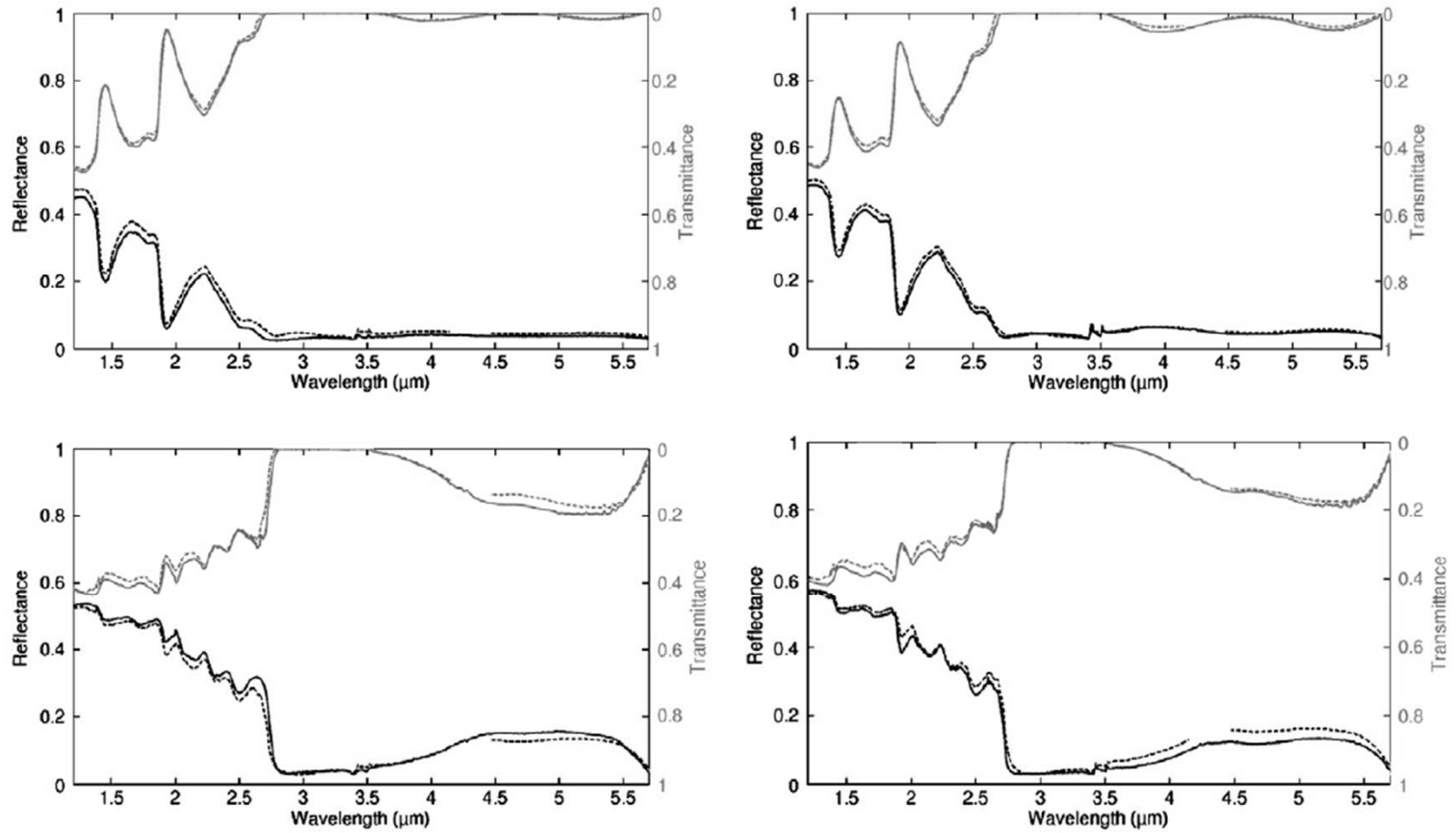
Fig. 10. Simulated (dashed line) vs. measured (plain line) reflectance and transmittance of fresh (top left: Catalpa , top right: Tillia ) and dry (bottom left: Catalpa , bottom right: Acer platanoides ) leaves.
