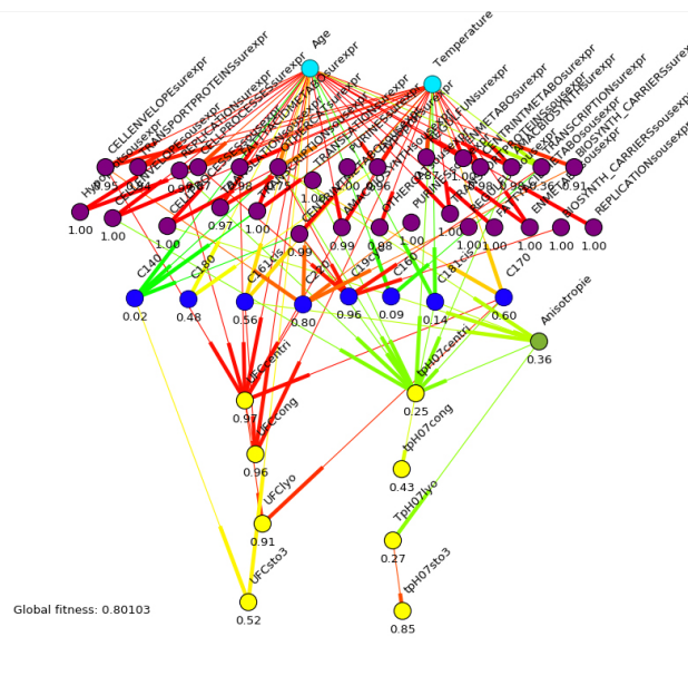
Fig. 4. Graphical model representing a global model. The Global fitness of the model is indicated at the bottom-left. The fitness value of each node is indicated under them.
