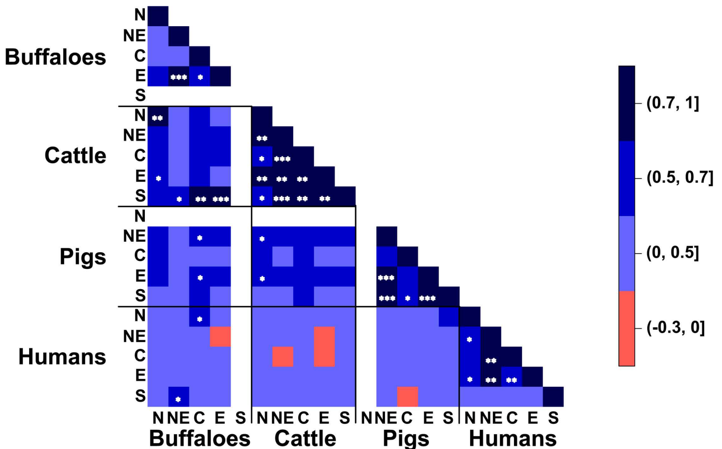
Fig 3. Spearman correlation of the pattern distributions of serovars between buffaloes, cattle, pigs and humans in northern (N), northeastern (NE), central (C), eastern (E), and southern (S) regions. * represents p-value < 0.05, ** represents p-value < 0.01, *** represents p-value < 0.001, and the white area represents correlation not available.
