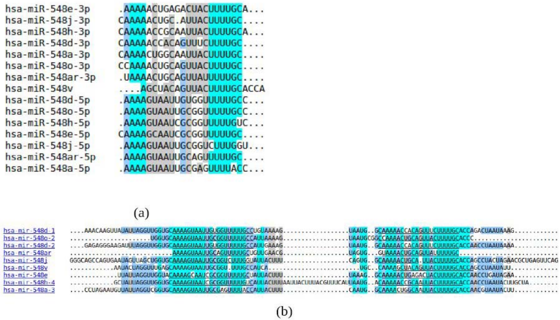
Figure 1 Alignments provided by miRBase for mir-548 family. Only sequences labeled as confident are given for miRNA (a) and pre-miRNA (b).
