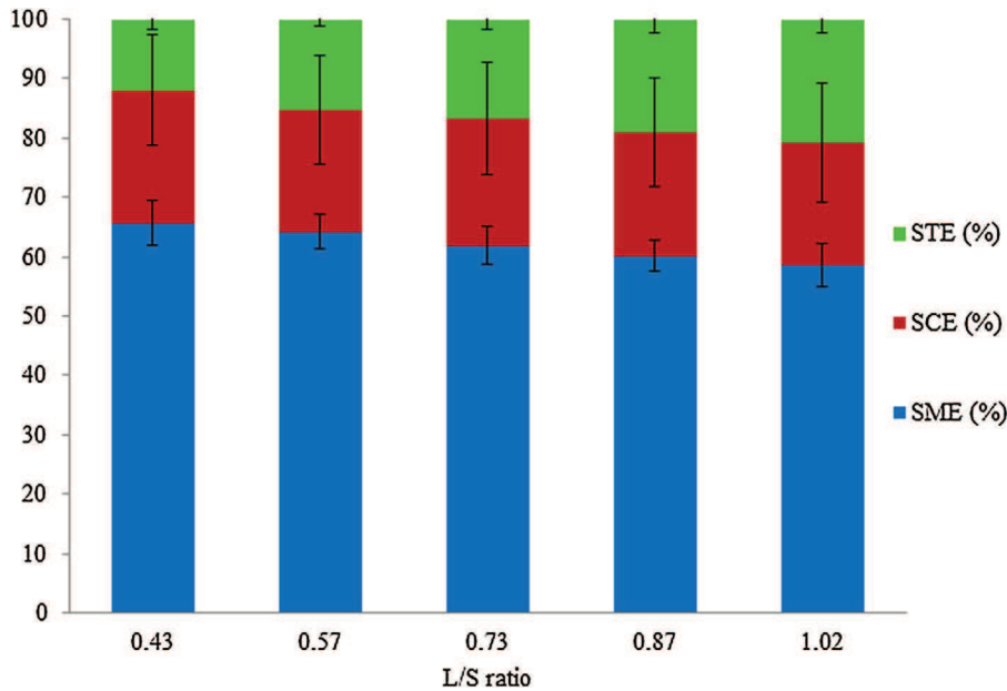
Fig. 2. Contribution of the three specific energy consumptions (%) in the Cleextral Evolum HT 53 twin-screw extruder as a function of L/S ratio.
