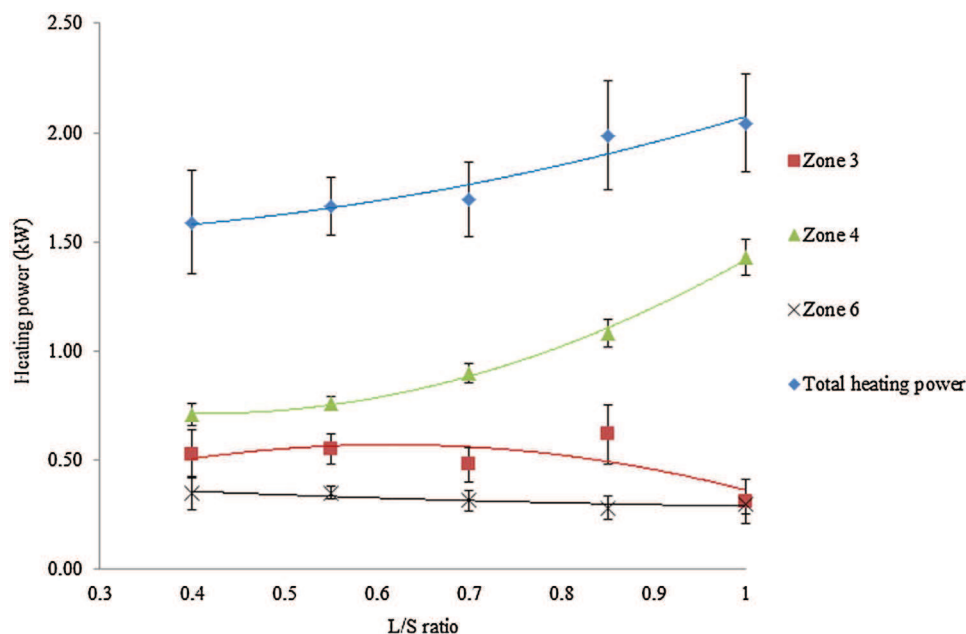
Fig. 3. Heating power along the barrel of the Cleextral Evolum HT 53 twin-screw extruder.
