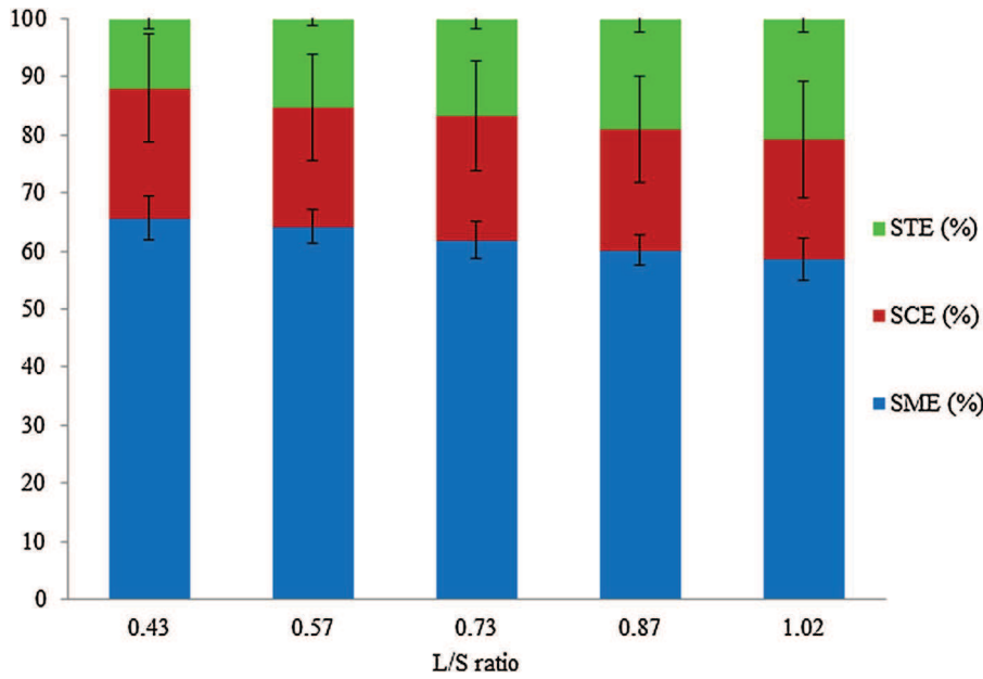
Fig. 2. Contribution of the three specific energy consumptions (%) in the Cleextral Evolum HT 53 twin-screw extruder as a function of L/S ratio.
