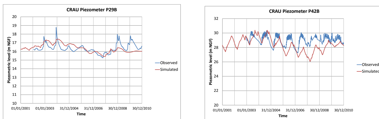
Figure 2 : comparison of measured and simulated piezometric levels in two wells of the Crau Plain .
