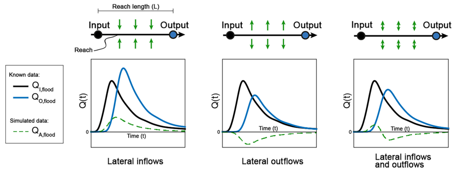
Figure 1. Diffusive wave equation to model lateral flood flow exchanges along a channel reach of length L . The black curve Q_{I,flood} depicts the evolution of the flow rate with time at the beginning of the channel (input), and the blue curve Q_{O,flood} at the end (output). The dashed green curve Q_{A,flood} corresponds to the lateral flow exchanges which are positive for lateral inflows or negative for lateral outflows.
