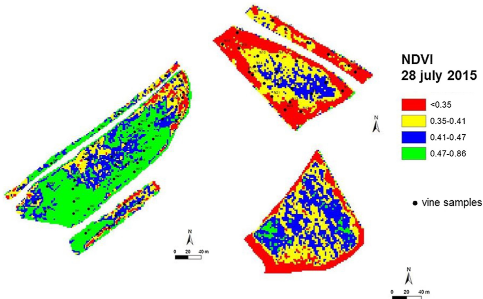
Fig. 7. Map of NDVI quartiles for the Pléiades image of 28 July 2015.
