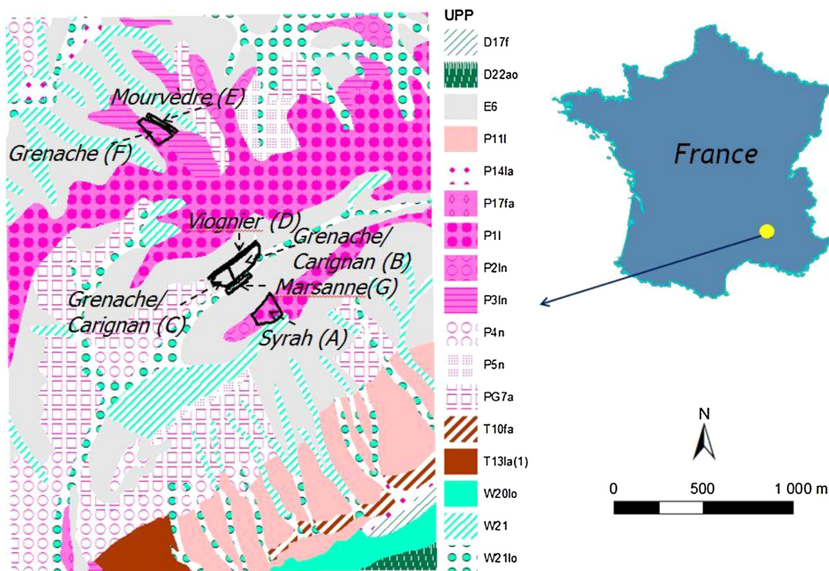
Fig. 1. General soil map derived from the regional soil landscape map (Vaudour et al., 1998; Vaudour, 2003), location of vine varieties within farm plots (in capital letters). D17f, D22ao: stagnic calcaric cambisols, fluvisols; E6, colluvic leptosols; P11l, P14la, colluvic pachic cambisols; P17fa, P1l, P2ln, P3ln, haplic/eutric skeletal petrocalcic cambisols (chromic); P4n, P5n, PG7a, colluvic, skeletal, anthrosols (escalic), petrocalcic calcisols; T10fa, T13la(1), chromic skeletal luvisols, cambisols; W20lo, W21, W21lo, skeletal fluvisols, colluvic regosols.
