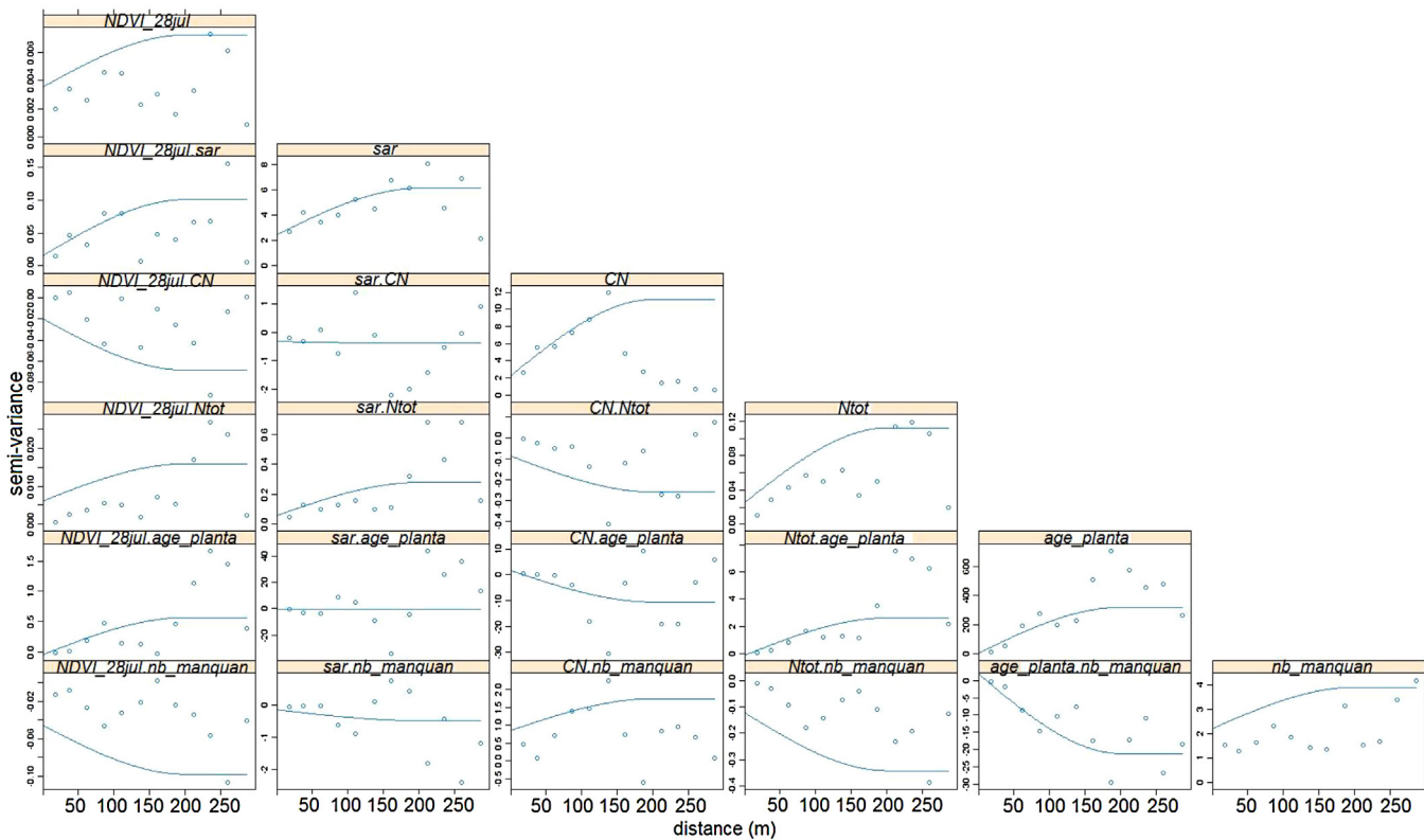
Fig. 13. Cross-variograms between the set of quantitative variables for the Grenache variety (49 samples, spherical model, range 200 m). sar, basal diameter of the bunch peduncle; CN, C/N ratio; Ntot, total nitrogen content; age_planta, planting age; nb_manquan, frequency of missing vines.
