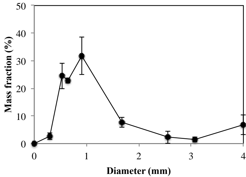
Fig. 3. Distribution curve of the diameters of the wet agglomerates processed by the fluidized bed (experiments using standard semolina and true water content of 0.37 g/g dry matter).
