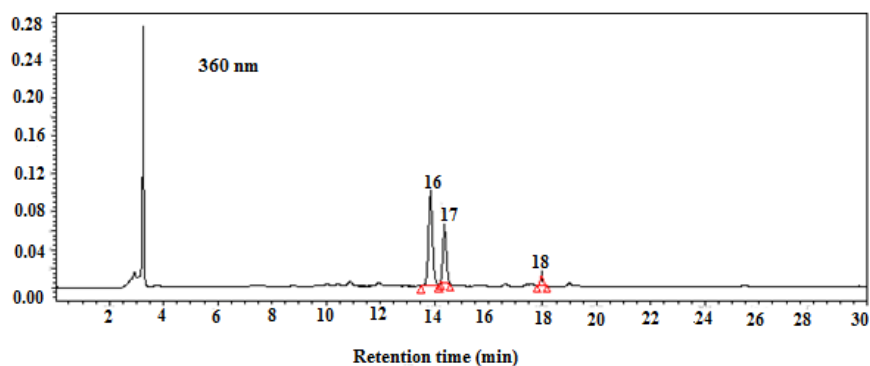
Figure 2. Flavonol chromatographic pattern of Gros noir (A), Cardinal (B) and Muscat noir (C) skin extract recorded at 360 nm. For list of substances, see Table 2.
