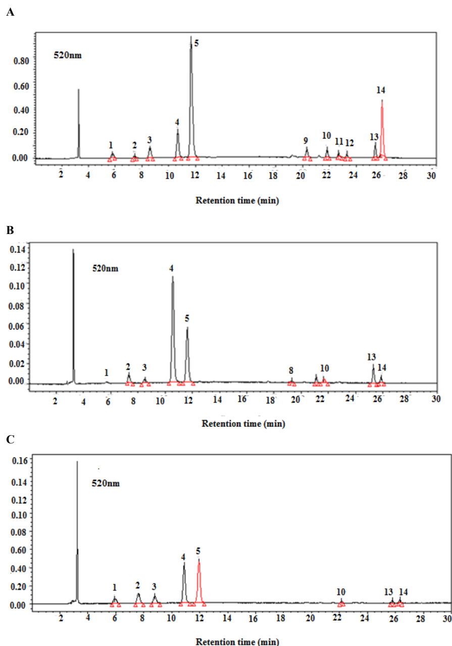
Figure 1 - Anthocyanin chromatographic pattern of Gros noir (A), Cardinal (B) and Muscat noir (C) skin extract recorded at 520 nm. For list of substances, see Table 2.
