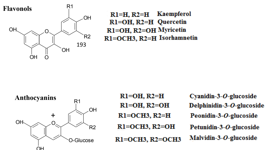
Figure 3 - Chemical structures of grape flavonols and anthocyanins.
